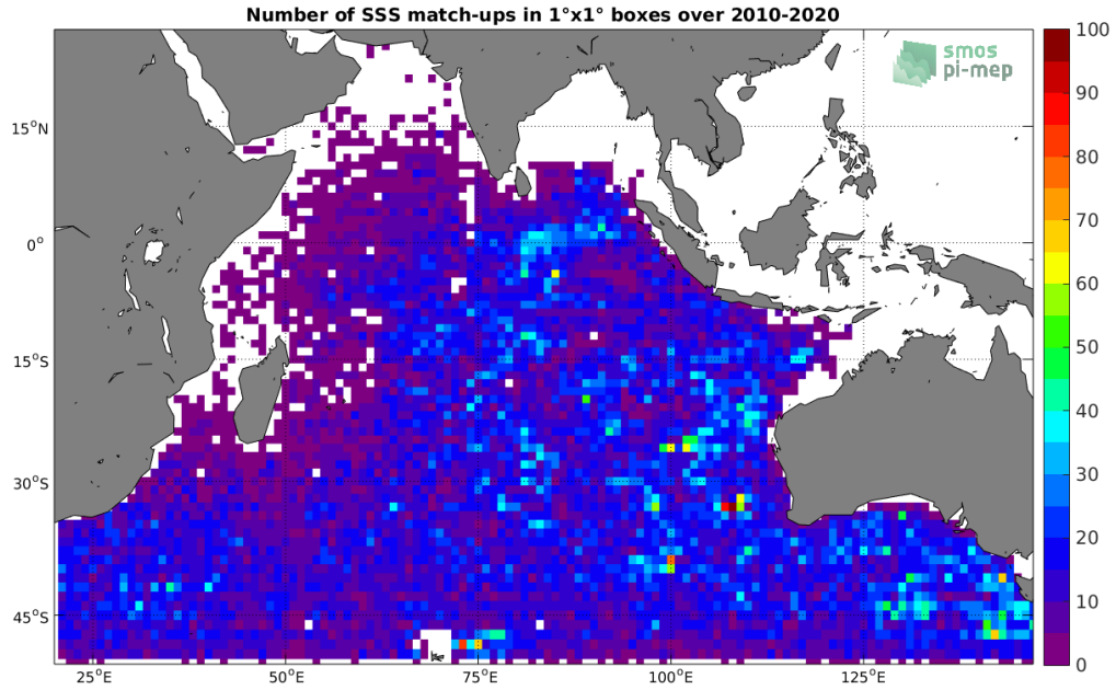
Figure 4: Number of SSS match-ups between Argo SSS and the SMOS SSS L2Q v321 - 0.25 Deg (CATDS-CPDC) SSS product for the Indian Ocean Pi-MEP region over 1°x1° boxes and for the full satellite product period.
