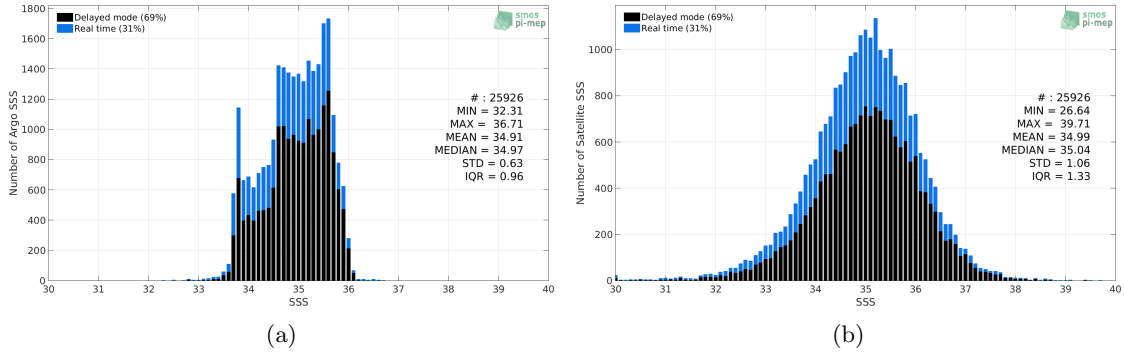
Figure 2: Histograms of SSS from Argo (a) and SMOS-L3-CATDS-CPDC-V321-L2Q (b) considering all match-up pairs per bins of 0.1 over the Indian Ocean Pi-MEP region and for the full satellite product period.
