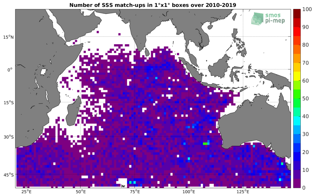
Figure 4: Number of SSS match-ups between Argo SSS and the SMOS-L3-CATDS-CPDC-V321-L2Q SSS product for the Indian Ocean Pi-MEP region over 1°x1° boxes and for the full satellite product period.
