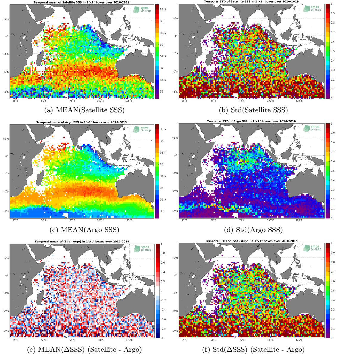
Figure 6: Temporal mean (left) and Std (right) of SSS from SMOS-L3-CATDS-CPDC-V321-L2Q (top), Argo (middle), and of \Delta SSS (Satellite - Argo). Only match-up pairs are used to generate these maps.
