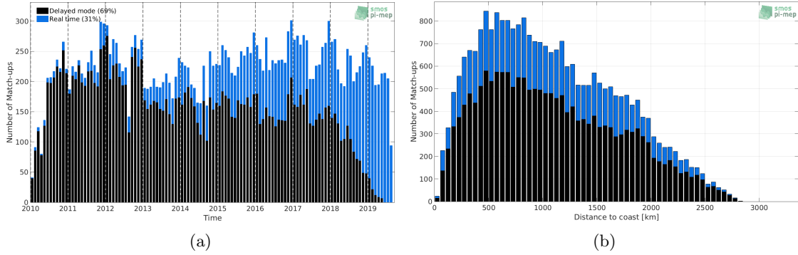
Figure 1: Number of match-ups between Argo and SMOS-L3-CATDS-CPDC-V321-L2Q SSS as a function of time (a) and as function of the distance to coast (b) over the Indian Ocean Pi-MEP region and for the full satellite product period.
