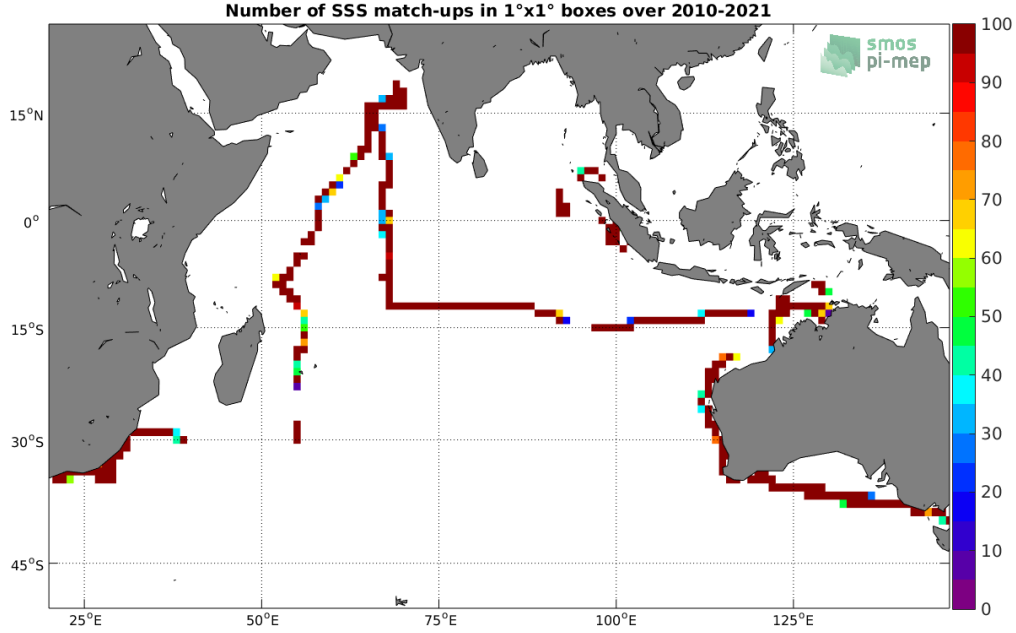
Figure 4: Number of SSS match-ups between TSG (SAMOS) SSS and the SMOS SSS L3 v317 - Monthly - 25 km (CATDS-CPDC) SSS product for the Indian Ocean Pi-MEP region over 1^\circ \times 1^\circ boxes and for the full satellite product period.
