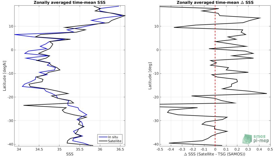
Figure 8: Left panel: Zonal mean SSS from SMOS SSS L3 v317 - Monthly - 25 km (CATDS-CPDC) satellite product (black) and from TSG (SAMOS) (blue). Right panel: Zonal mean of \Delta\text{SSS} (Satellite - TSG (SAMOS)) for all the collected Pi-MEP match-up pairs estimated over the full satellite product period.
