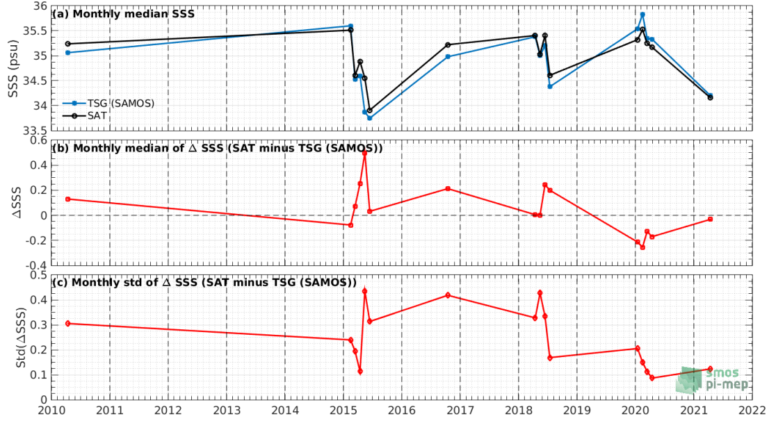
Figure 7: Time series of the monthly median SSS (top), median of \Delta\text{SSS} (Satellite - TSG (SAMOS)) and Std of \Delta\text{SSS} (Satellite - TSG (SAMOS)) over the Indian Ocean Pi-MEP region considering all match-ups collected by the Pi-MEP.
