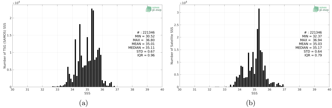
Figure 2: Histograms of SSS from TSG (SAMOS) (a) and SMOS SSS L3 v317 - Monthly - 25 km (CATDS-CPDC) (b) considering all match-up pairs per bins of 0.1 over the Indian Ocean Pi-MEP region and for the full satellite product period.
