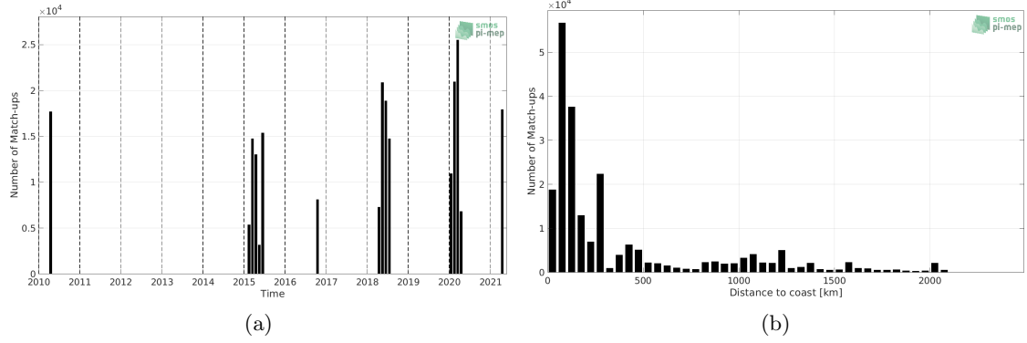
Figure 1: Number of match-ups between TSG (SAMOS) and SMOS SSS L3 v317 - Monthly - 25 km (CATDS-CPDC) SSS as a function of time (a) and as function of the distance to coast (b) over the Indian Ocean Pi-MEP region and for the full satellite product period.
