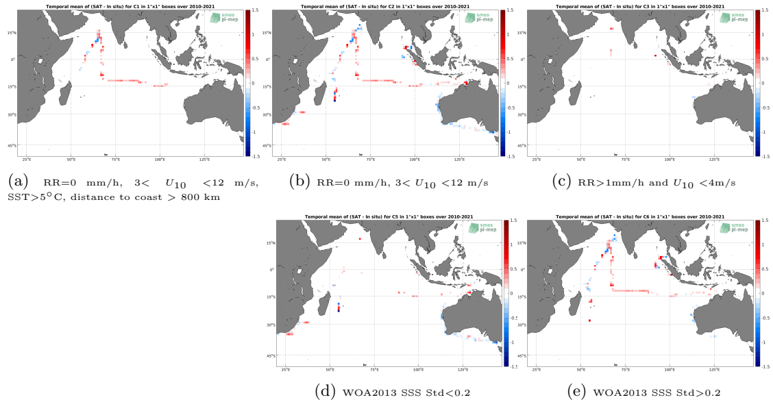
Figure 12: Temporal mean gridded over spatial boxes of size 1^\circ \times 1^\circ of \Delta SSS (SMOS SSS L3 v317 - Monthly - 25 km (CATDS-CPDC) - TSG (SAMOS)) for 5 different subdatasets corresponding to: RR=0 mm/h, 3 < U_{10} < 12 m/s, SST > 5^\circ\text{C} , distance to coast > 800 km (a), RR=0 mm/h, 3 < U_{10} < 12 m/s (b), RR > 1 mm/h and U_{10} < 4 m/s (c), WOA2013 SSS Std < 0.2 (d), WOA2013 SSS Std > 0.2 (e).
