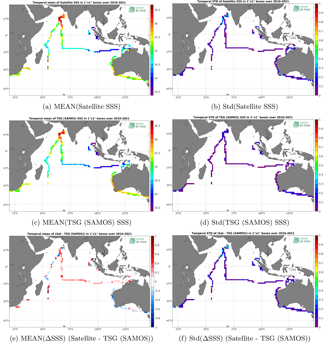
Figure 6: Temporal mean (left) and Std (right) of SSS from SMOS SSS L3 v317 - Monthly - 25 km (CATDS-CPDC) (top), TSG (SAMOS) (middle), and of \Delta SSS (Satellite - TSG (SAMOS)). Only match-up pairs are used to generate these maps.
