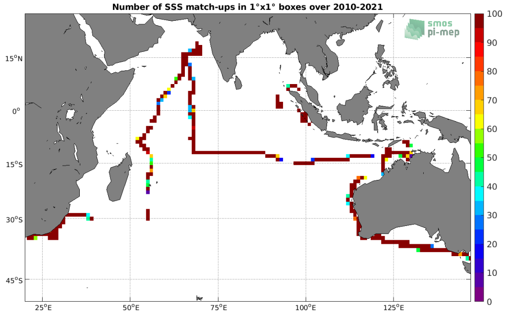
Figure 4: Number of SSS match-ups between TSG (SAMOS) SSS and the SMOS SSS L3 v317 - Monthly - 25 km (CATDS-CPDC) SSS product for the Indian Ocean Pi-MEP region over 1^\circ \times 1^\circ boxes and for the full satellite product period.
