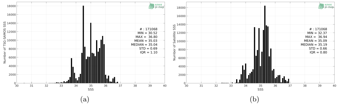
Figure 2: Histograms of SSS from TSG-SAMOS (a) and SMOS L3 v317 - Monthly - 25 km (CATDS-CPDC) (b) considering all match-up pairs per bins of 0.1 over the Indian Ocean Pi-MEP region and for the full satellite product period.
