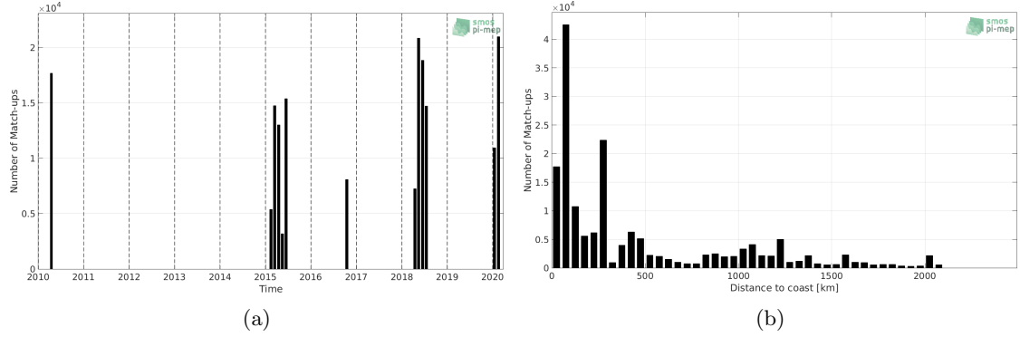
Figure 1: Number of match-ups between TSG-SAMOS and SMOS L3 v317 - Monthly - 25 km (CATDS-CPDC) SSS as a function of time (a) and as function of the distance to coast (b) over the Indian Ocean Pi-MEP region and for the full satellite product period.
