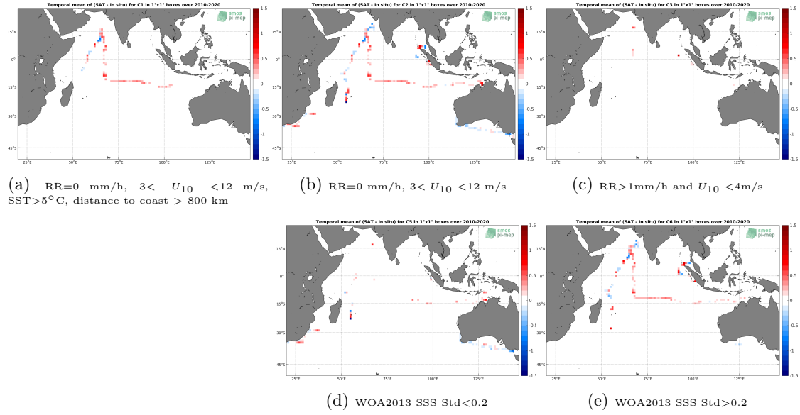
Figure 12: Temporal mean gridded over spatial boxes of size 1^\circ \times 1^\circ of \Delta SSS (SMOS L3 v317 - Monthly - 25 km (CATDS-CPDC) - TSG-SAMOS) for 5 different subdatasets corresponding to: RR=0 mm/h, 3 < U_{10} < 12 m/s, SST >5^\circ C, distance to coast > 800 km (a), RR=0 mm/h, 3 < U_{10} < 12 m/s (b), RR >1 mm/h and U_{10} < 4 m/s (c), WOA2013 SSS Std <0.2 (d), WOA2013 SSS Std >0.2 (e).
