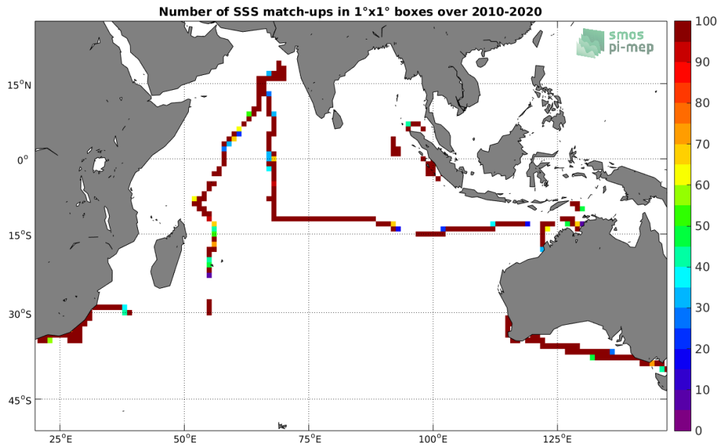
Figure 4: Number of SSS match-ups between TSG-SAMOS SSS and the SMOS L3 v317 - Monthly - 25 km (CATDS-CPDC) SSS product for the Indian Ocean Pi-MEP region over 1^\circ \times 1^\circ boxes and for the full satellite product period.
