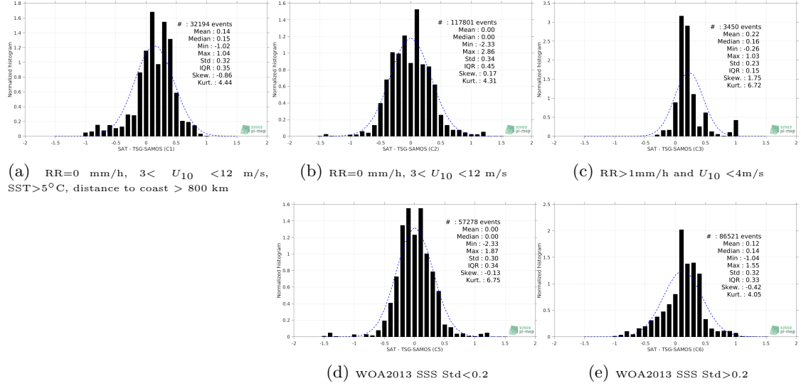
Figure 13: Normalized histogram of \Delta SSS (SMOS L3 v317 - Monthly - 25 km (CATDS-CPDC) - TSG-SAMOS) for 5 different subdatasets corresponding to: RR=0 mm/h, 3 < U_{10} < 12 m/s, SST > 5^\circ C , distance to coast > 800 km (a), RR=0 mm/h, 3 < U_{10} < 12 m/s (b), RR > 1 mm/h and U_{10} < 4 m/s (c), WOA2013 SSS Std < 0.2 (d), WOA2013 SSS Std > 0.2 (e).
