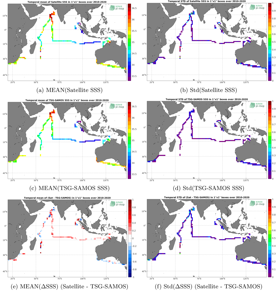
Figure 6: Temporal mean (left) and Std (right) of SSS from SMOS L3 v317 - Monthly - 25 km (CATDS-CPDC) (top), TSG-SAMOS (middle), and of \Delta SSS (Satellite - TSG-SAMOS). Only match-up pairs are used to generate these maps.
