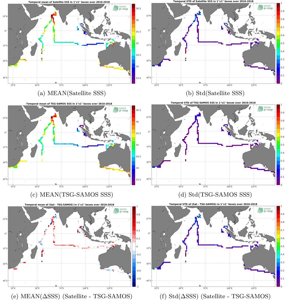
Figure 6: Temporal mean (left) and Std (right) of SSS from SMOS-L3-CATDS-CPDC-V317-MONTHLY-25KM (top), TSG-SAMOS (middle), and of \Delta SSS (Satellite - TSG-SAMOS). Only match-up pairs are used to generate these maps.
