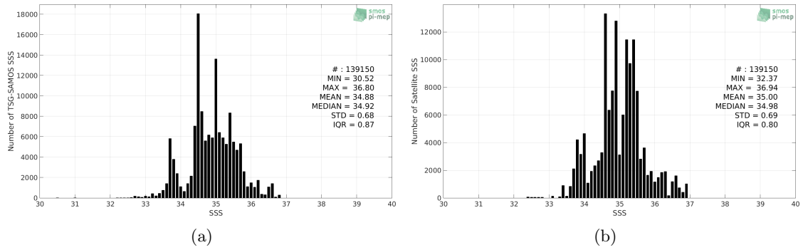
Figure 2: Histograms of SSS from TSG-SAMOS (a) and SMOS-L3-CATDS-CPDC-V317-MONTHLY-25KM (b) considering all match-up pairs per bins of 0.1 over the Indian Ocean Pi-MEP region and for the full satellite product period.
