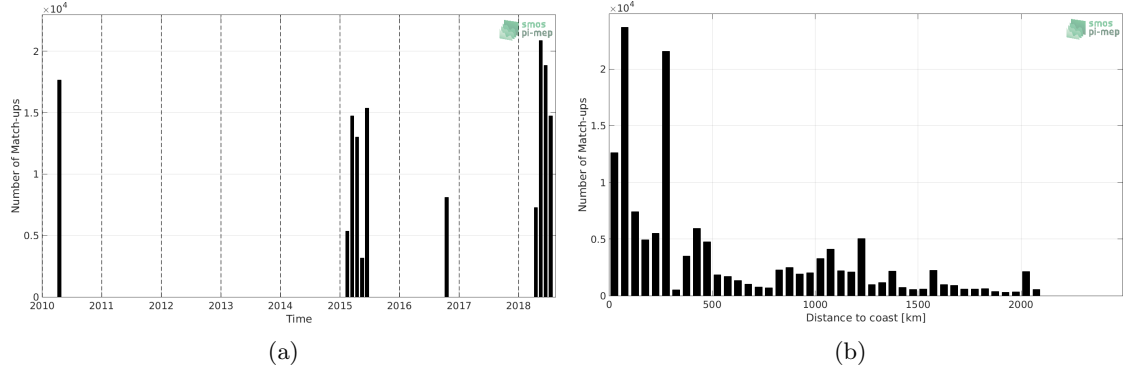
Figure 1: Number of match-ups between TSG-SAMOS and SMOS-L3-CATDS-CPDC-V317-MONTHLY-25KM SSS as a function of time (a) and as function of the distance to coast (b) over the Indian Ocean Pi-MEP region and for the full satellite product period.
