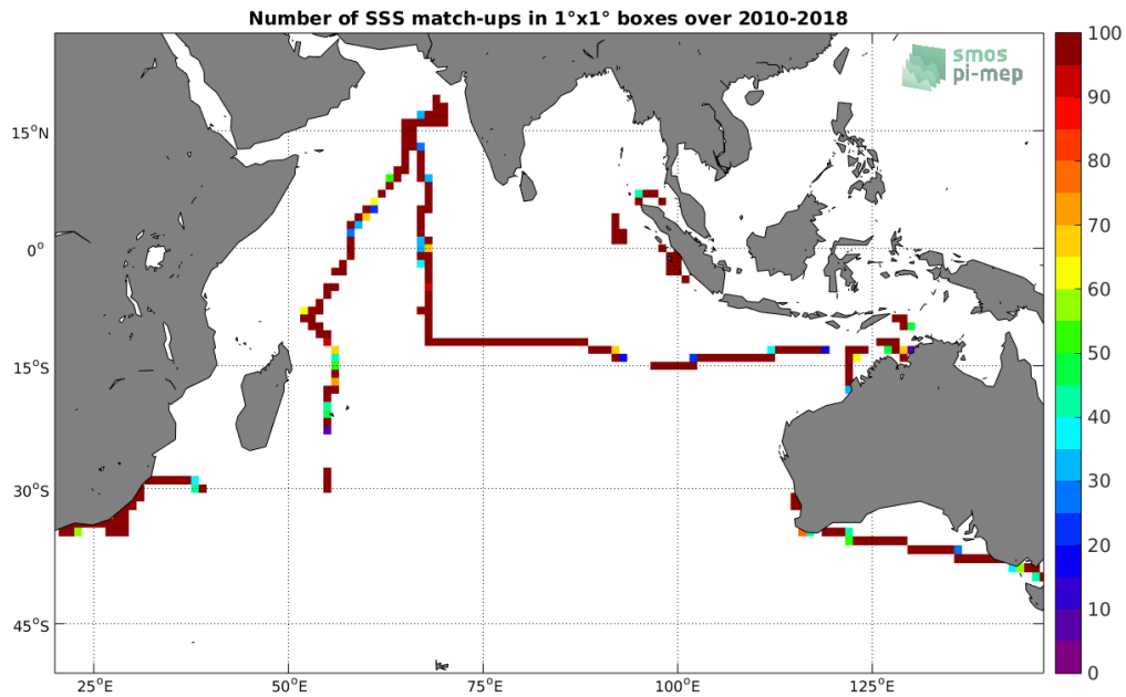
Figure 4: Number of SSS match-ups between TSG-SAMOS SSS and the SMOS-L3-CATDS-CPDC-V317-MONTHLY-25KM SSS product for the Indian Ocean Pi-MEP region over 1^\circ \times 1^\circ boxes and for the full satellite product period.
