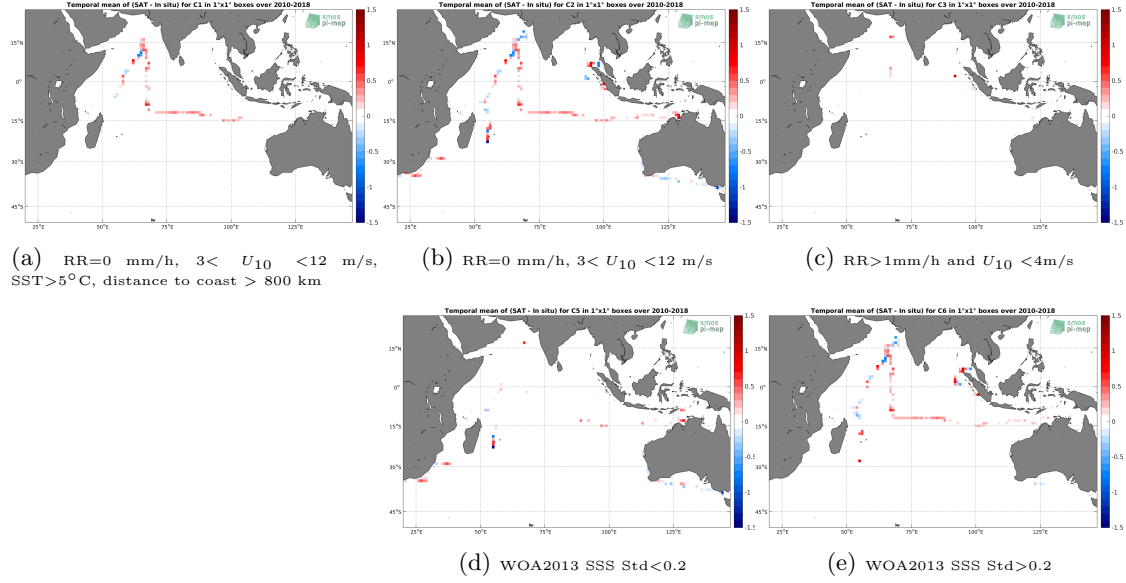
Figure 12: Temporal mean gridded over spatial boxes of size 1^\circ \times 1^\circ of \Delta SSS (SMOS-L3-CATDS-CPDC-V317-MONTHLY-25KM - TSG-SAMOS) for 5 different subdatasets corresponding to: RR=0 mm/h, 3 < U_{10} < 12 m/s, SST > 5^\circ C , distance to coast > 800 km (a), RR=0 mm/h, 3 < U_{10} < 12 m/s (b), RR > 1 mm/h and U_{10} < 4 m/s (c), WOA2013 SSS Std < 0.2 (d), WOA2013 SSS Std > 0.2 (e).
