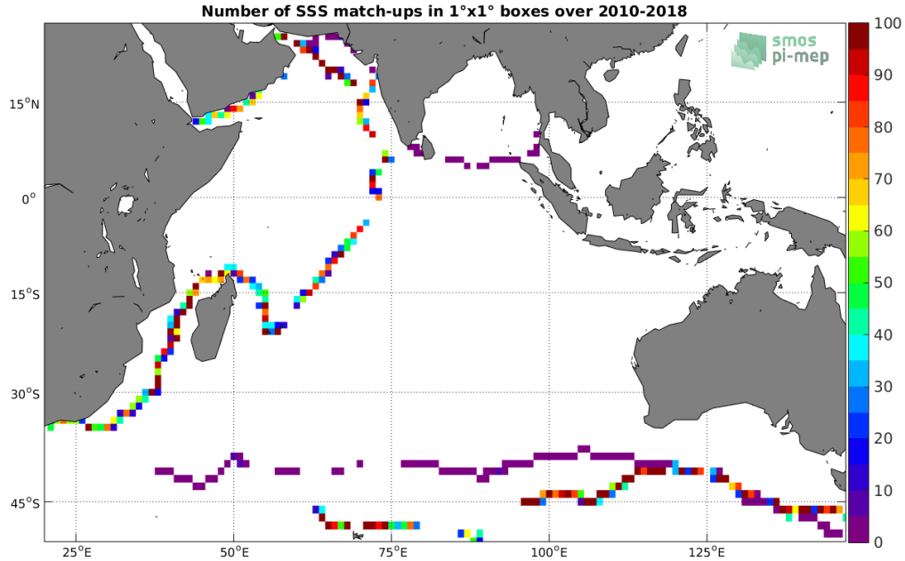
Figure 4: Number of SSS match-ups between TSG (GOSUD-Sailing-ship) SSS and the SMOS SSS L3 v317 - Monthly - 25 km (CATDS-CPDC) SSS product for the Indian Ocean Pi-MEP region over 1^\circ \times 1^\circ boxes and for the full satellite product period.
