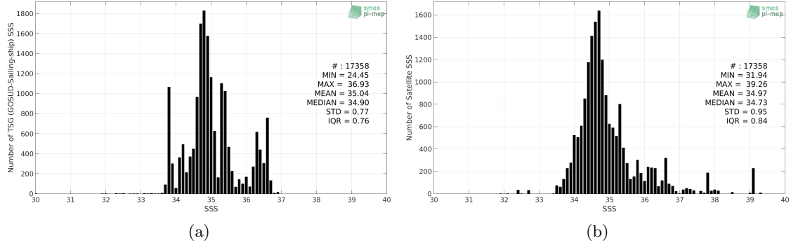
Figure 2: Histograms of SSS from TSG (GOSUD-Sailing-ship) (a) and SMOS SSS L3 v317 - Monthly - 25 km (CATDS-CPDC) (b) considering all match-up pairs per bins of 0.1 over the Indian Ocean Pi-MEP region and for the full satellite product period.
