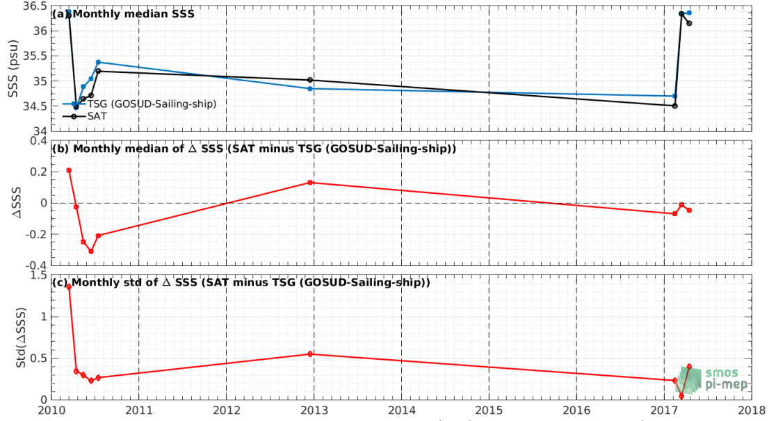
Figure 7: Time series of the monthly median SSS (top), median of \Delta\text{SSS} (Satellite - TSG (GOSUD-Sailing-ship)) and Std of \Delta\text{SSS} (Satellite - TSG (GOSUD-Sailing-ship)) over the Indian Ocean Pi-MEP region considering all match-ups collected by the Pi-MEP.
