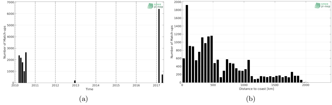
Figure 1: Number of match-ups between TSG (GOSUD-Sailing-ship) and SMOS SSS L3 v317 - Monthly - 25 km (CATDS-CPDC) SSS as a function of time (a) and as function of the distance to coast (b) over the Indian Ocean Pi-MEP region and for the full satellite product period.
