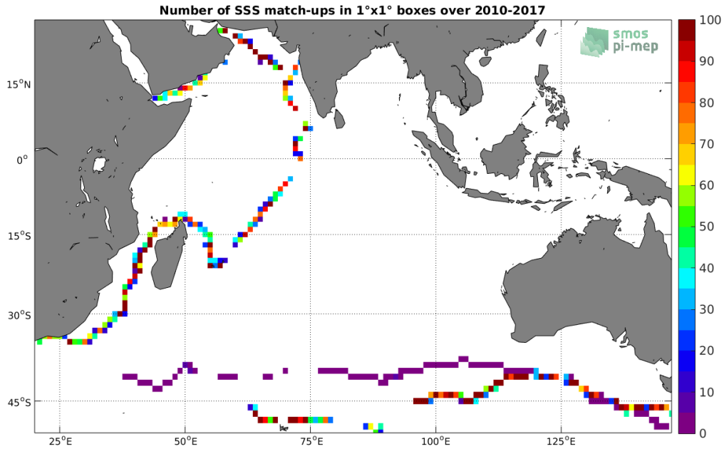
Figure 4: Number of SSS match-ups between TSG (GOSUD-Sailing-ship) SSS and the SMOS SSS L3 v317 - Monthly - 25 km (CATDS-CPDC) SSS product for the Indian Ocean Pi-MEP region over 1°x1° boxes and for the full satellite product period.
