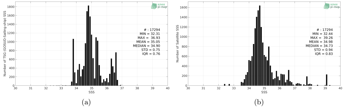
Figure 2: Histograms of SSS from TSG (GOSUD-Sailing-ship) (a) and SMOS SSS L3 v317 - Monthly - 25 km (CATDS-CPDC) (b) considering all match-up pairs per bins of 0.1 over the Indian Ocean Pi-MEP region and for the full satellite product period.
