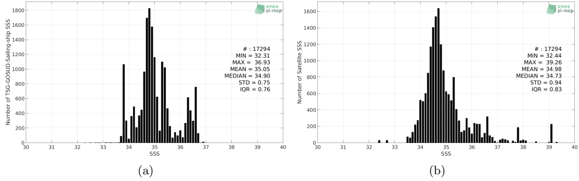
Figure 2: Histograms of SSS from TSG-GOSUD-Sailing-ship (a) and SMOS L3 v317 - Monthly - 25 km (CATDS-CPDC) (b) considering all match-up pairs per bins of 0.1 over the Indian Ocean Pi-MEP region and for the full satellite product period.
