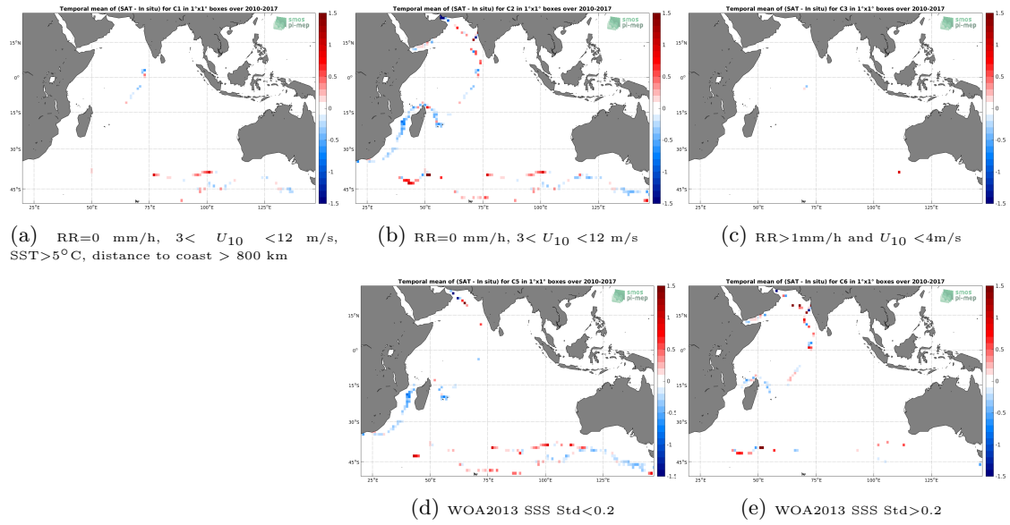
Figure 12: Temporal mean gridded over spatial boxes of size 1^\circ \times 1^\circ of \Delta SSS (SMOS L3 v317 - Monthly - 25 km (CATDS-CPDC) - TSG-GOSUD-Sailing-ship) for 5 different subdatasets corresponding to: RR=0 mm/h, 3 < U_{10} < 12 m/s, SST > 5^\circ C , distance to coast > 800 km (a), RR=0 mm/h, 3 < U_{10} < 12 m/s (b), RR > 1 mm/h and U_{10} < 4 m/s (c), WOA2013 SSS Std < 0.2 (d), WOA2013 SSS Std > 0.2 (e).
