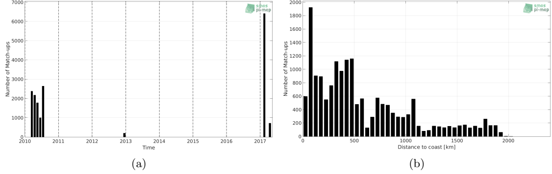
Figure 1: Number of match-ups between TSG-GOSUD-Sailing-ship and SMOS L3 v317 - Monthly - 25 km (CATDS-CPDC) SSS as a function of time (a) and as function of the distance to coast (b) over the Indian Ocean Pi-MEP region and for the full satellite product period.
