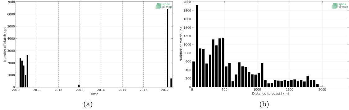
Figure 1: Number of match-ups between TSG-GOSUD-Sailing-ship and SMOS-L3-CATDS-CPDC-V317-MONTHLY-25KM SSS as a function of time (a) and as function of the distance to coast (b) over the Indian Ocean Pi-MEP region and for the full satellite product period.
