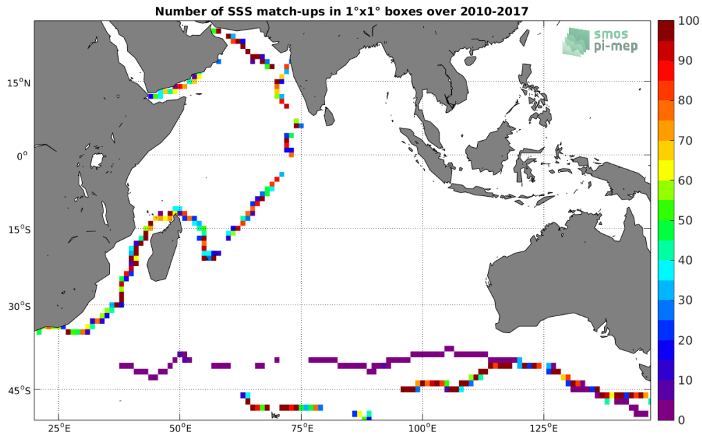
Figure 4: Number of SSS match-ups between TSG-GOSUD-Sailing-ship SSS and the SMOS-L3-CATDS-CPDC-V317-MONTHLY-25KM SSS product for the Indian Ocean Pi-MEP region over 1°x1° boxes and for the full satellite product period.
