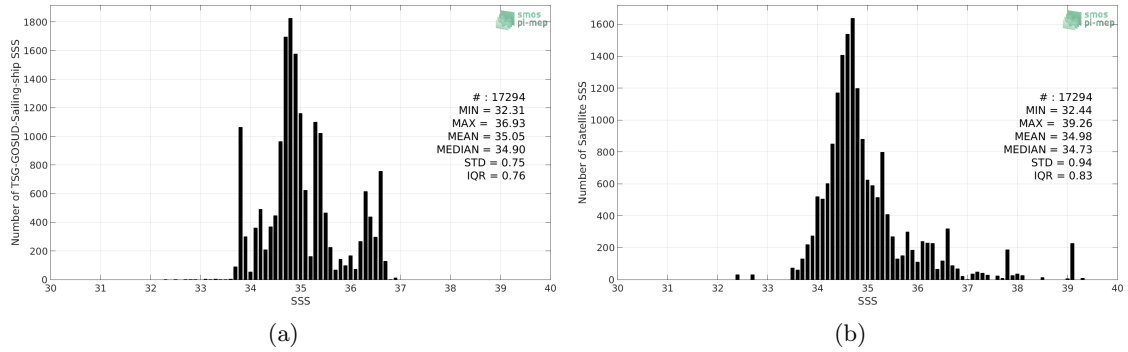
Figure 2: Histograms of SSS from TSG-GOSUD-Sailing-ship (a) and SMOS-L3-CATDS-CPDC-V317-MONTHLY-25KM (b) considering all match-up pairs per bins of 0.1 over the Indian Ocean Pi-MEP region and for the full satellite product period.
