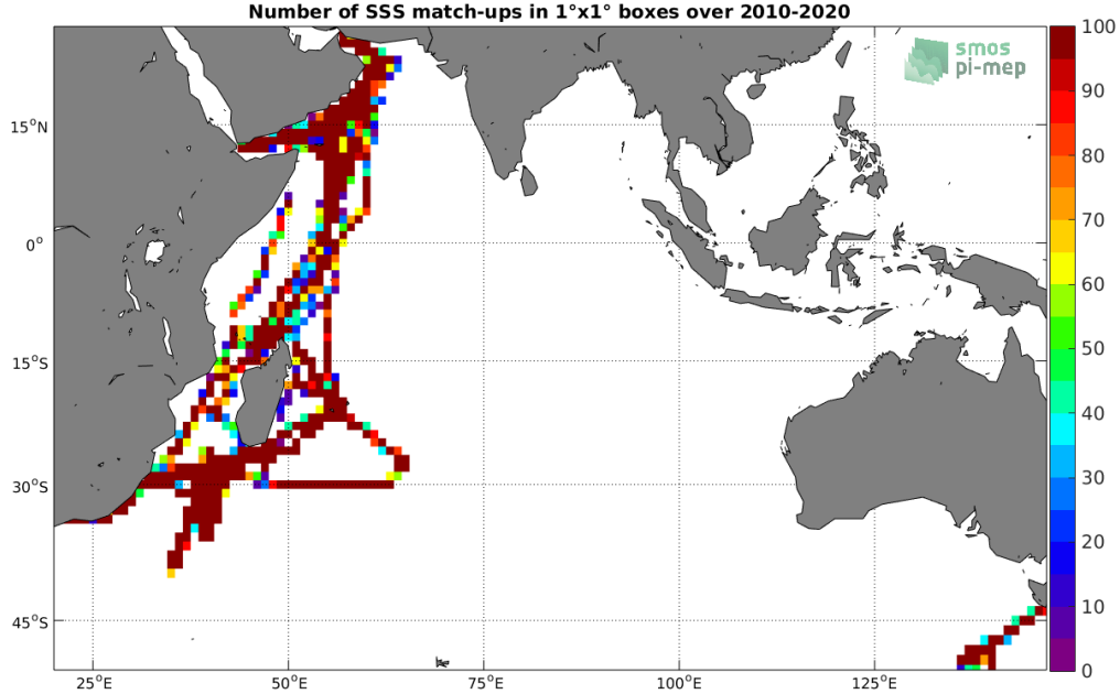
Figure 4: Number of SSS match-ups between TSG (GOSUD-Research-vessel) SSS and the SMOS SSS L3 v317 - Monthly - 25 km (CATDS-CPDC) SSS product for the Indian Ocean Pi-MEP region over 1^\circ \times 1^\circ boxes and for the full satellite product period.
