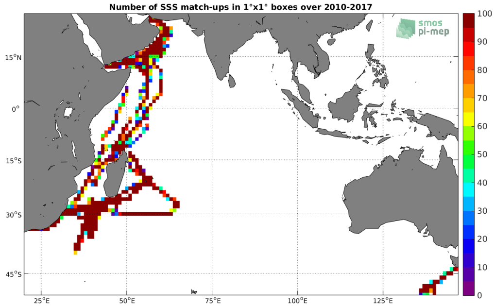
Figure 4: Number of SSS match-ups between TSG (GOSUD-Research-vessel) SSS and the SMOS SSS L3 v317 - Monthly - 25 km (CATDS-CPDC) SSS product for the Indian Ocean Pi-MEP region over 1°x1° boxes and for the full satellite product period.
