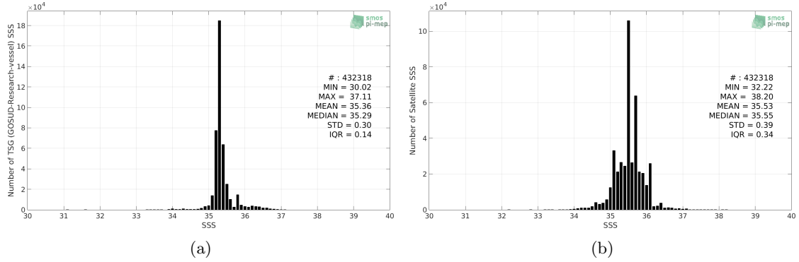
Figure 2: Histograms of SSS from TSG (GOSUD-Research-vessel) (a) and SMOS SSS L3 v317 - Monthly - 25 km (CATDS-CPDC) (b) considering all match-up pairs per bins of 0.1 over the Indian Ocean Pi-MEP region and for the full satellite product period.
