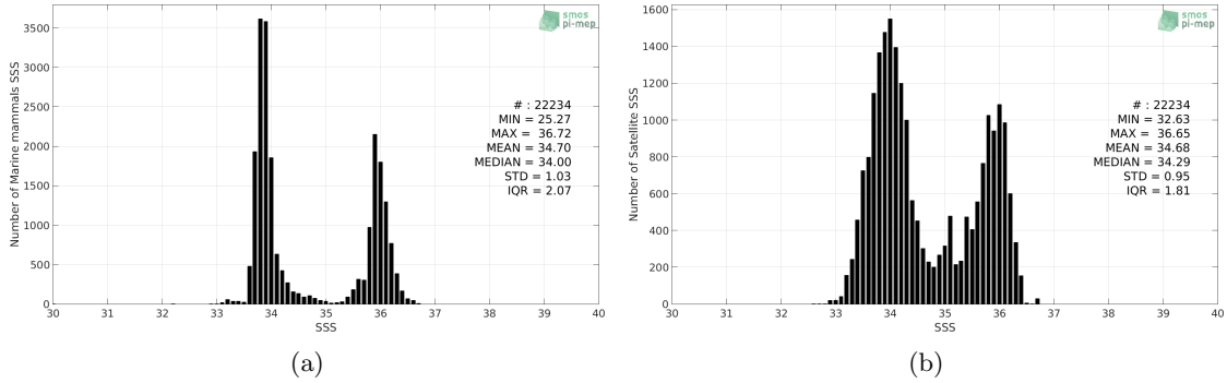
Figure 2: Histograms of SSS from Marine mammals (a) and SMOS SSS L3 v317 - Monthly - 25 km (CATDS-CPDC) (b) considering all match-up pairs per bins of 0.1 over the Indian Ocean Pi-MEP region and for the full satellite product period.
