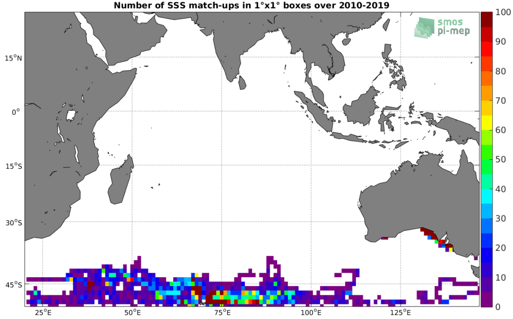
Figure 4: Number of SSS match-ups between Marine mammals SSS and the SMOS SSS L3 v317 - Monthly - 25 km (CATDS-CPDC) SSS product for the Indian Ocean Pi-MEP region over 1^\circ \times 1^\circ boxes and for the full satellite product period.
