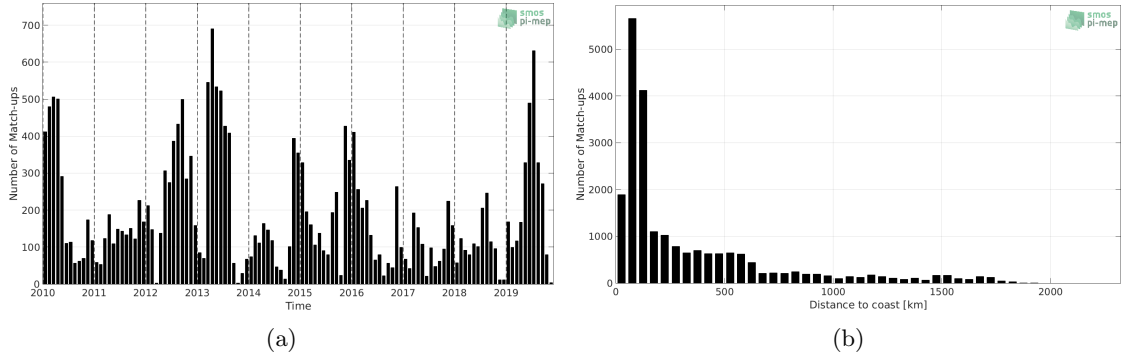
Figure 1: Number of match-ups between Marine mammals and SMOS SSS L3 v317 - Monthly - 25 km (CATDS-CPDC) SSS as a function of time (a) and as function of the distance to coast (b) over the Indian Ocean Pi-MEP region and for the full satellite product period.
