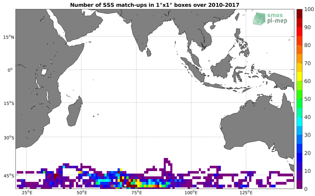
Figure 4: Number of SSS match-ups between Sea mammals SSS and the SMOS SSS L3 v317 - Monthly - 25 km (CATDS-CPDC) SSS product for the Indian Ocean Pi-MEP region over 1°x1° boxes and for the full satellite product period.
