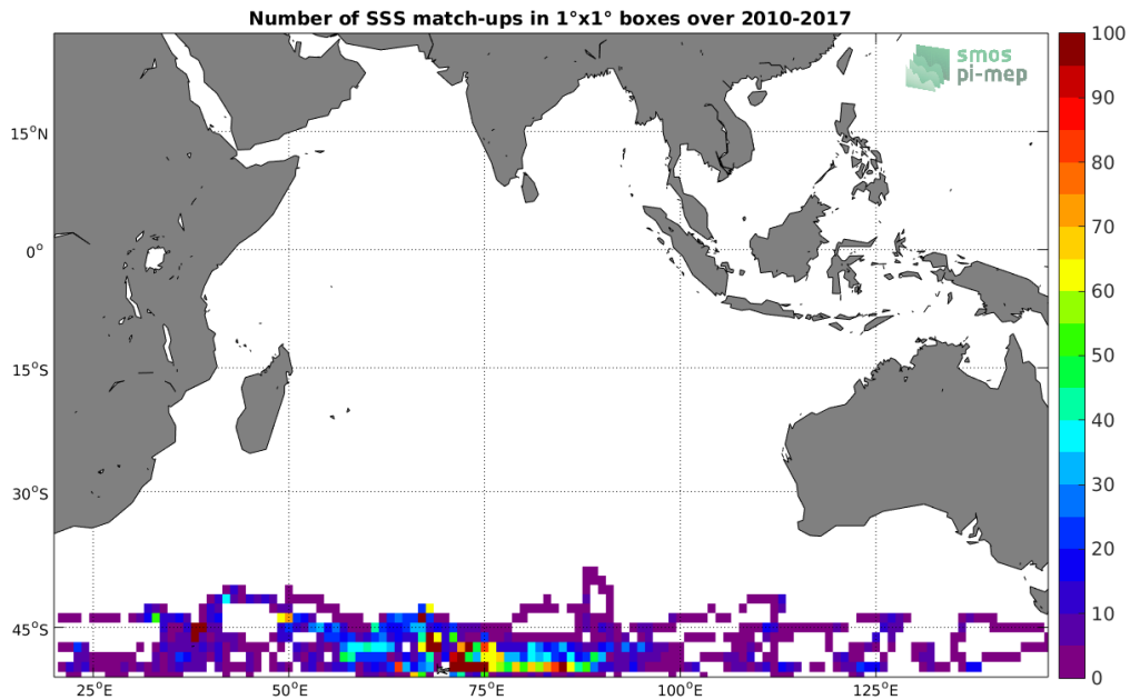
Figure 4: Number of SSS match-ups between Sea mammals SSS and the SMOS SSS L3 v317 - Monthly - 25 km (CATDS-CPDC) SSS product for the Indian Ocean Pi-MEP region over 1°x1° boxes and for the full satellite product period.
