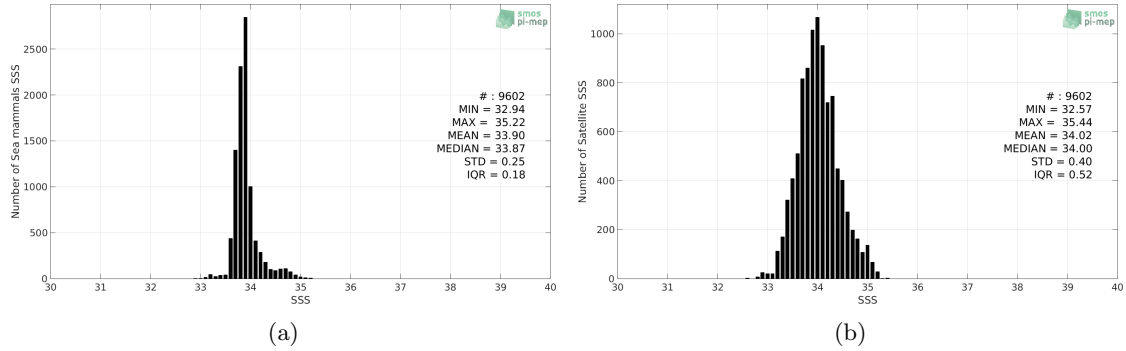
Figure 2: Histograms of SSS from Sea mammals (a) and SMOS SSS L3 v317 - Monthly - 25 km (CATDS-CPDC) (b) considering all match-up pairs per bins of 0.1 over the Indian Ocean Pi-MEP region and for the full satellite product period.
