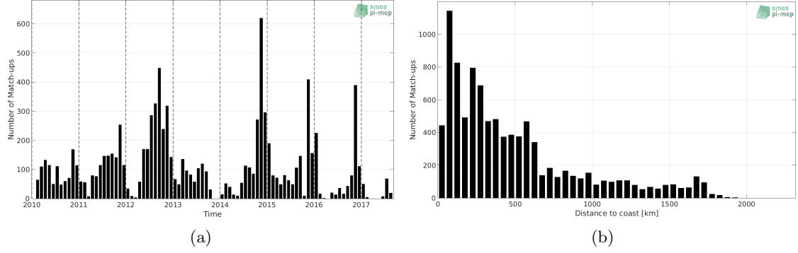
Figure 1: Number of match-ups between Sea mammals and SMOS SSS L3 v317 - Monthly - 25 km (CATDS-CPDC) SSS as a function of time (a) and as function of the distance to coast (b) over the Indian Ocean Pi-MEP region and for the full satellite product period.
