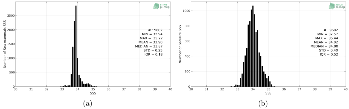
Figure 2: Histograms of SSS from Sea mammals (a) and SMOS L3 v317 - Monthly - 25 km (CATDS-CPDC) (b) considering all match-up pairs per bins of 0.1 over the Indian Ocean Pi-MEP region and for the full satellite product period.
