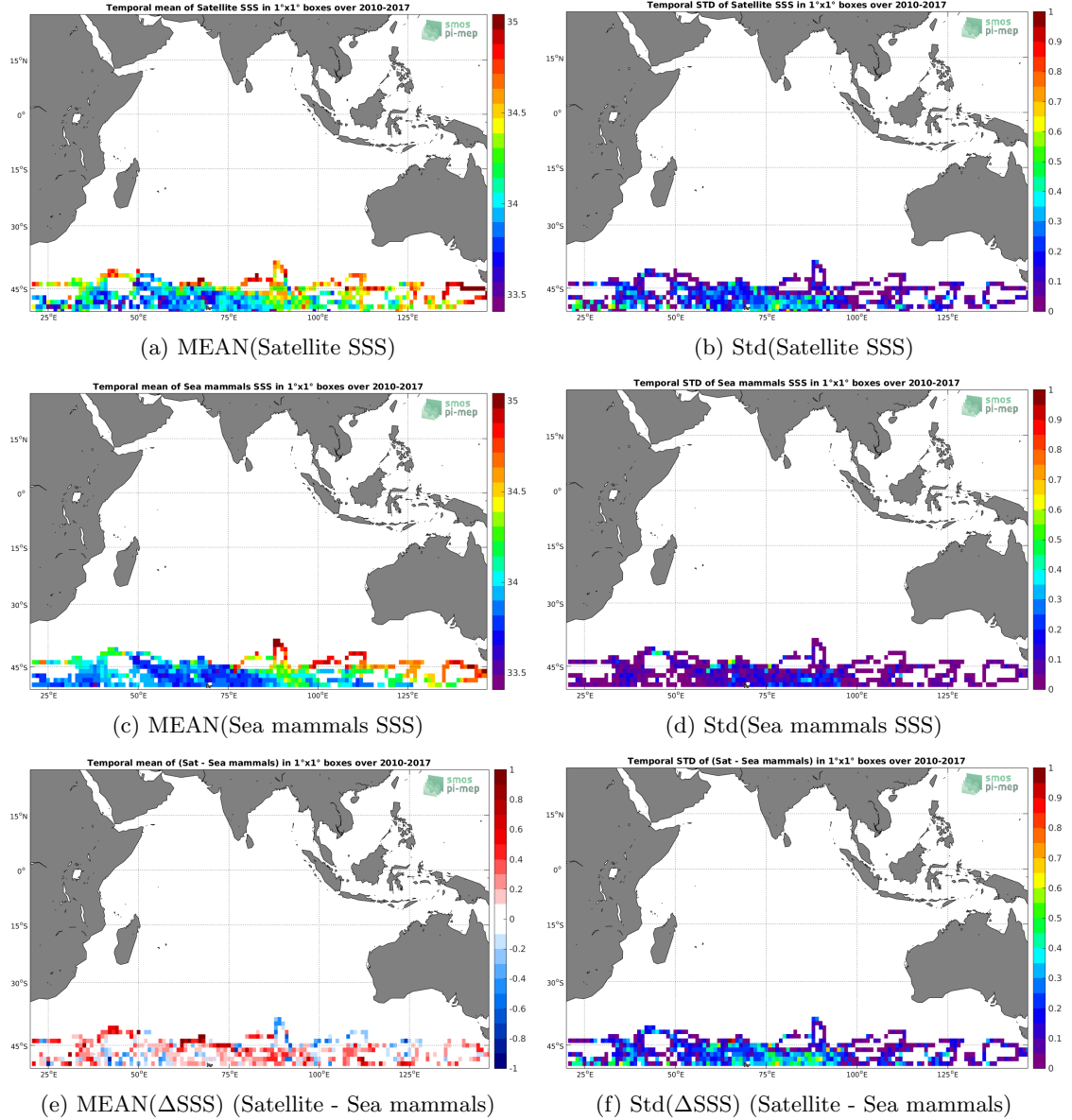
Figure 6: Temporal mean (left) and Std (right) of SSS from SMOS L3 v317 - Monthly - 25 km (CATDS-CPDC) (top), Sea mammals (middle), and of \Delta SSS (Satellite - Sea mammals). Only match-up pairs are used to generate these maps.
