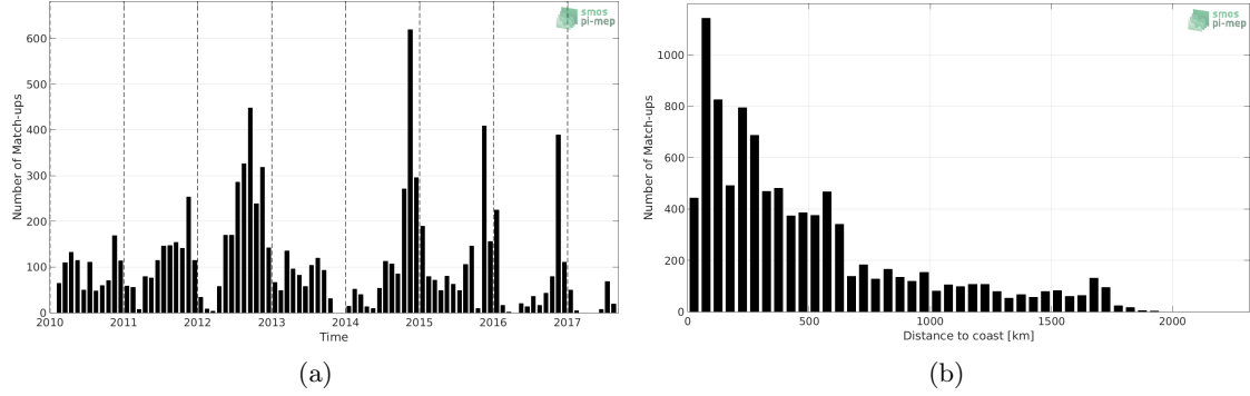
Figure 1: Number of match-ups between Sea mammals and SMOS L3 v317 - Monthly - 25 km (CATDS-CPDC) SSS as a function of time (a) and as function of the distance to coast (b) over the Indian Ocean Pi-MEP region and for the full satellite product period.
