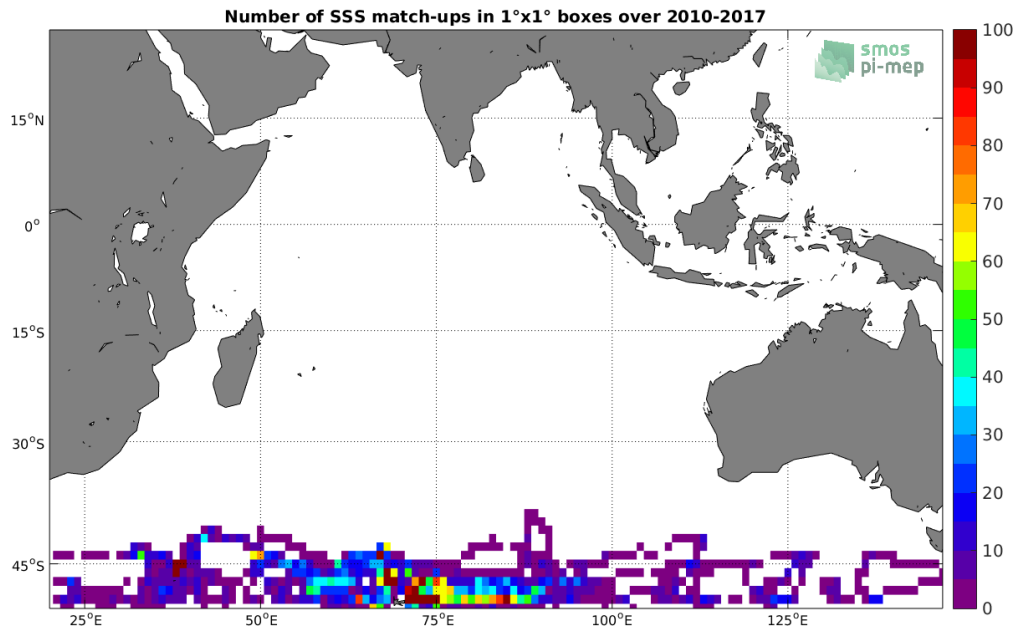
Figure 4: Number of SSS match-ups between Sea mammals SSS and the SMOS L3 v317 - Monthly - 25 km (CATDS-CPDC) SSS product for the Indian Ocean Pi-MEP region over 1°x1° boxes and for the full satellite product period.
