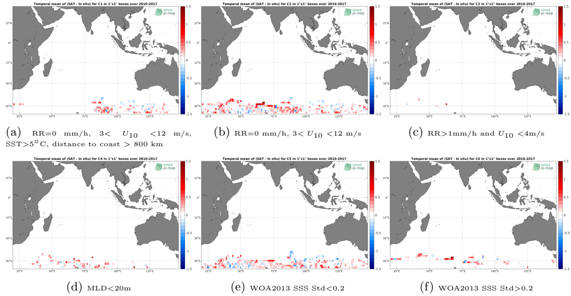
Figure 12: Temporal mean gridded over spatial boxes of size 1^{\circ}\times 1^{\circ} of \Delta\text{SSS} (SMOS L3 v317 - Monthly - 25 km (CATDS-CPDC) - Sea mammals) for 6 different subdatasets corresponding to: \text{RR}=0 mm/h, 3 < U_{10} < 12 m/s, SST > 5^{\circ}\text{C} , distance to coast > 800 km (a), \text{RR}=0 mm/h, 3 < U_{10} < 12 m/s (b), \text{RR} > 1\text{mm/h} and U_{10} < 4\text{m/s} (c), \text{MLD} < 20\text{m} (d), WOA2013 SSS Std < 0.2 (e), WOA2013 SSS Std > 0.2 (f).
