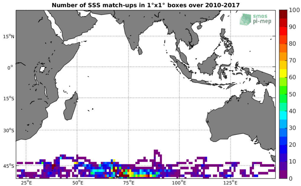
Figure 4: Number of SSS match-ups between Sea mammals SSS and the SMOS-L3-CATDS-CPDC-V317-MONTHLY-25KM SSS product for the Indian Ocean Pi-MEP region over 1^\circ \times 1^\circ boxes and for the full satellite product period.
