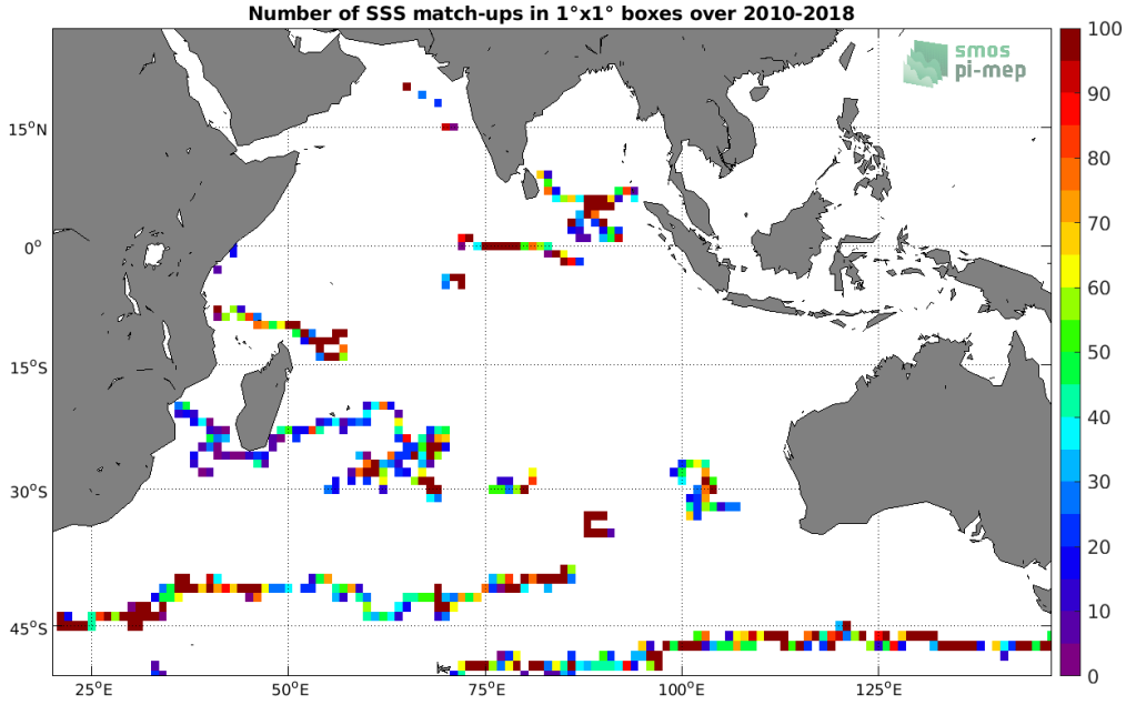
Figure 3: Number of SSS match-ups between Surface drifters SSS and the SMOS SSS L3 v317 - Monthly - 25 km (CATDS-CPDC) SSS product for the Indian Ocean Pi-MEP region over 1^\circ \times 1^\circ boxes and for the full satellite product period.
