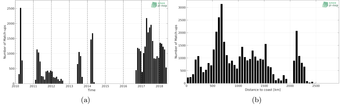
Figure 1: Number of match-ups between Surface drifters and SMOS SSS L3 v317 - Monthly - 25 km (CATDS-CPDC) SSS as a function of time (a) and as function of the distance to coast (b) over the Indian Ocean Pi-MEP region and for the full satellite product period.
