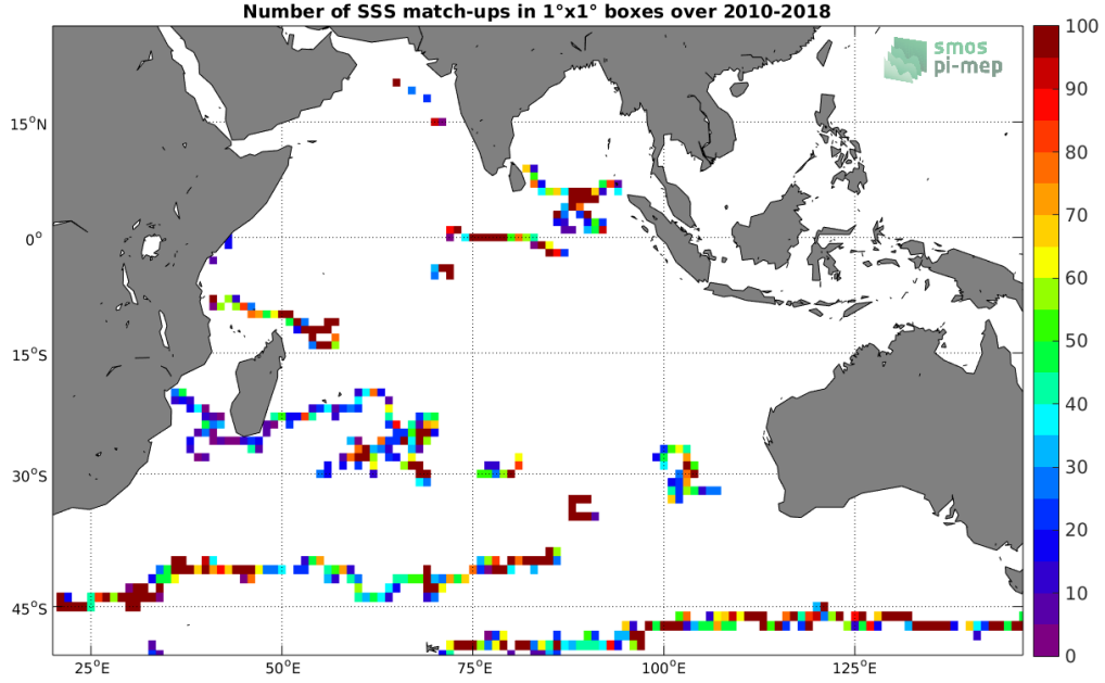
Figure 3: Number of SSS match-ups between Surface drifters SSS and the SMOS SSS L3 v317 - Monthly - 25 km (CATDS-CPDC) SSS product for the Indian Ocean Pi-MEP region over 1^\circ \times 1^\circ boxes and for the full satellite product period.
