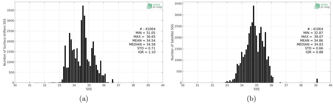
Figure 2: Histograms of SSS from Surface drifters (a) and SMOS SSS L3 v317 - Monthly - 25 km (CATDS-CPDC) (b) considering all match-up pairs per bins of 0.1 over the Indian Ocean Pi-MEP region and for the full satellite product period.
