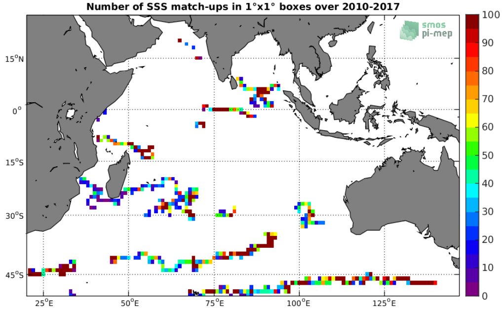
Figure 3: Number of SSS match-ups between Surface drifters SSS and the SMOS-L3-CATDS-CPDC-V317-MONTHLY-25KM SSS product for the Indian Ocean Pi-MEP region over 1^\circ \times 1^\circ boxes and for the full satellite product period.
