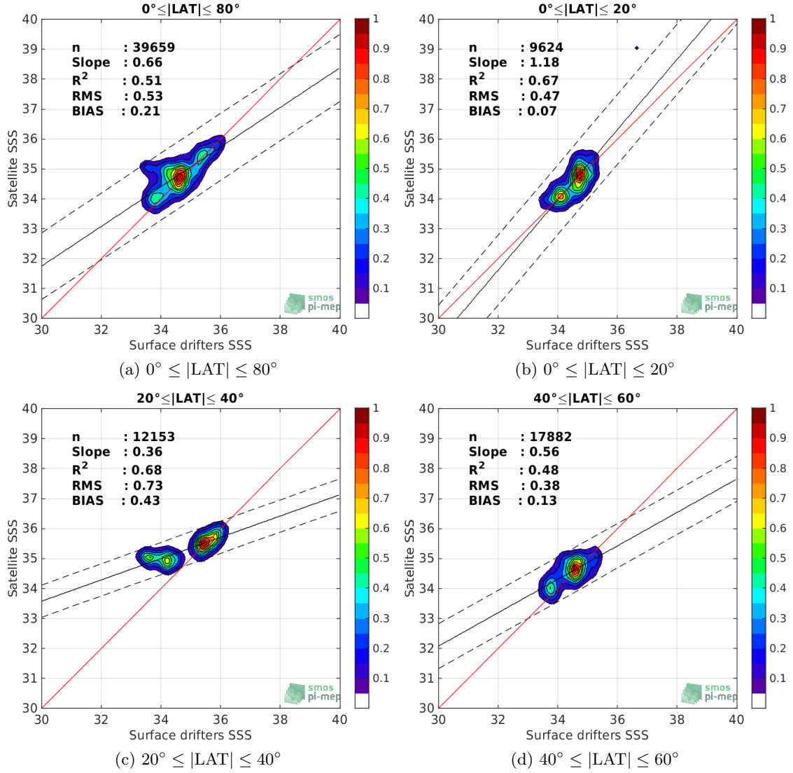
Figure 8: Contour maps of the concentration of SMOS-L3-CATDS-CPDC-V317-MONTHLY-25KM SSS (y-axis) versus Surface drifters SSS (x-axis) at match-up pairs for different latitude bands. For each plot, the red line shows x=y . The black thin and dashed lines indicate a linear fit through the data cloud and the \pm 95\% confidence levels, respectively. The number match-up pairs n , the slope and R^2 coefficient of the linear fit, the root mean square (RMS) and the mean bias between satellite and in situ data are indicated for each latitude band in each plot.
