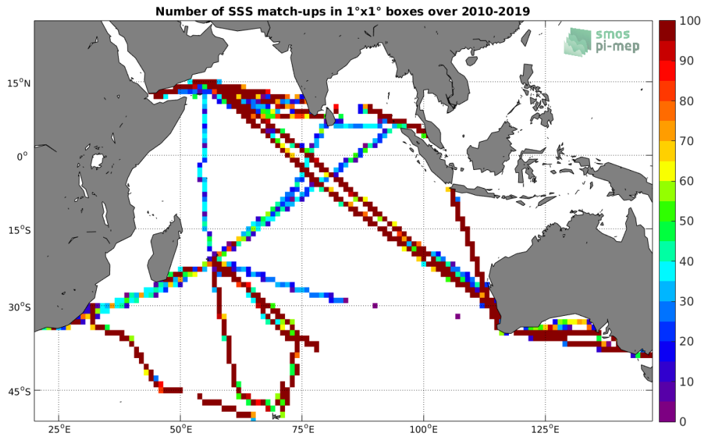
Figure 4: Number of SSS match-ups between TSG (LEGOS-DM) SSS and the SMOS SSS L3 v317 - 10 Days - 25 km (CATDS-CPDC) SSS product for the Indian Ocean Pi-MEP region over 1^\circ \times 1^\circ boxes and for the full satellite product period.
