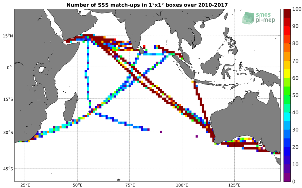
Figure 4: Number of SSS match-ups between TSG-LEGOS-DM SSS and the SMOS-L3-CATDS-CPDC-V317-10DAYS-25KM SSS product for the Indian Ocean Pi-MEP region over 1^\circ \times 1^\circ boxes and for the full satellite product period.
