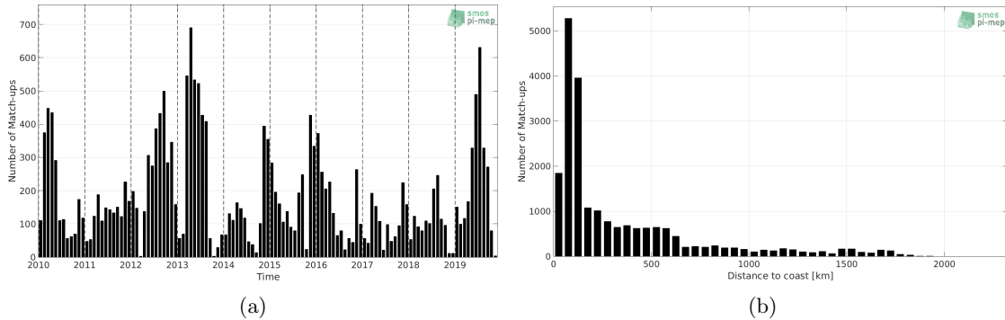
Figure 1: Number of match-ups between Marine mammals and SMOS SSS L3 v317 - 10 Days - 25 km (CATDS-CPDC) SSS as a function of time (a) and as function of the distance to coast (b) over the Indian Ocean Pi-MEP region and for the full satellite product period.
