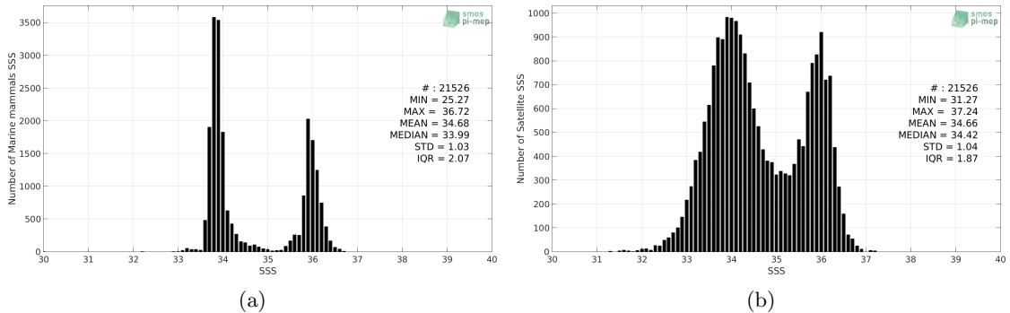
Figure 2: Histograms of SSS from Marine mammals (a) and SMOS SSS L3 v317 - 10 Days - 25 km (CATDS-CPDC) (b) considering all match-up pairs per bins of 0.1 over the Indian Ocean Pi-MEP region and for the full satellite product period.
