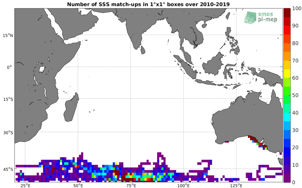
Figure 4: Number of SSS match-ups between Marine mammals SSS and the SMOS SSS L3 v317 - 10 Days - 25 km (CATDS-CPDC) SSS product for the Indian Ocean Pi-MEP region over 1^\circ \times 1^\circ boxes and for the full satellite product period.
