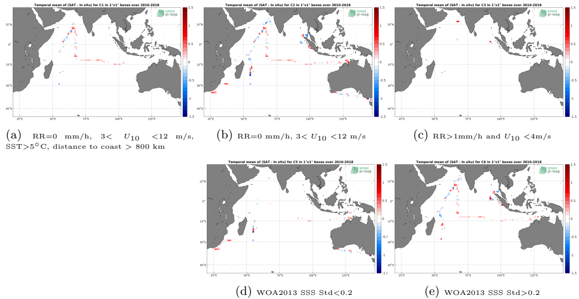
Figure 12: Temporal mean gridded over spatial boxes of size 1^\circ \times 1^\circ of \Delta SSS (SMOS-L3-CATDS-CPDC-V3-MONTHLY-25KM - TSG-SAMOS) for 5 different subdatasets corresponding to:RR=0 mm/h, 3 < U_{10} < 12 m/s, SST >5^\circ C, distance to coast > 800 km (a), RR=0 mm/h, 3 < U_{10} < 12 m/s (b), RR >1 mm/h and U_{10} < 4 m/s (c), WOA2013 SSS Std <0.2 (d), WOA2013 SSS Std >0.2 (e).
