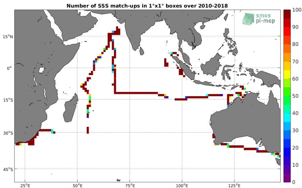
Figure 4: Number of SSS match-ups between TSG-SAMOS SSS and the SMOS-L3-CATDS-CPDC-V3-MONTHLY-25KM SSS product for the Indian Ocean Pi-MEP region over 1^\circ \times 1^\circ boxes and for the full satellite product period.
