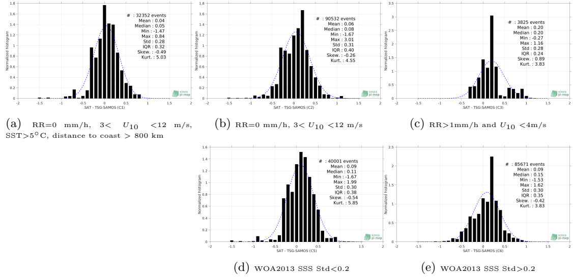
Figure 13: Normalized histogram of \Delta SSS (SMOS-L3-CATDS-CPDC-V3-MONTHLY-25KM - TSG-SAMOS) for 5 different subdatasets corresponding to: RR=0 mm/h, 3 < U_{10} < 12 m/s, SST > 5°C, distance to coast > 800 km (a), RR=0 mm/h, 3 < U_{10} < 12 m/s (b), RR > 1mm/h and U_{10} < 4 m/s (c), WOA2013 SSS Std < 0.2 (d), WOA2013 SSS Std > 0.2 (e).
