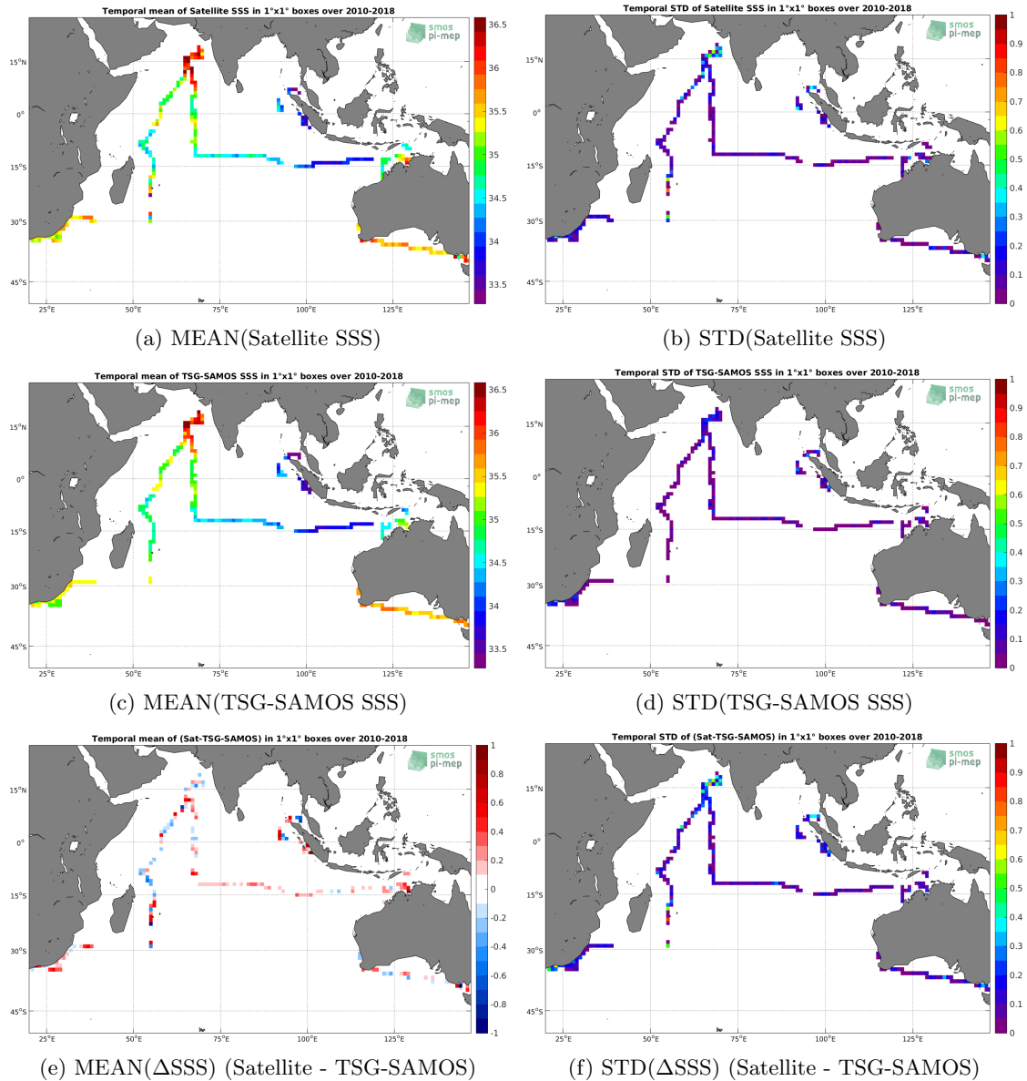
Figure 6: Temporal mean (left) and STD (right) of SSS from SMOS-L3-CATDS-CPDC-V3-MONTHLY-25KM (top), TSG-SAMOS (middle), and of \Delta SSS (Satellite - TSG-SAMOS). Only match-up pairs are used to generate these maps.
