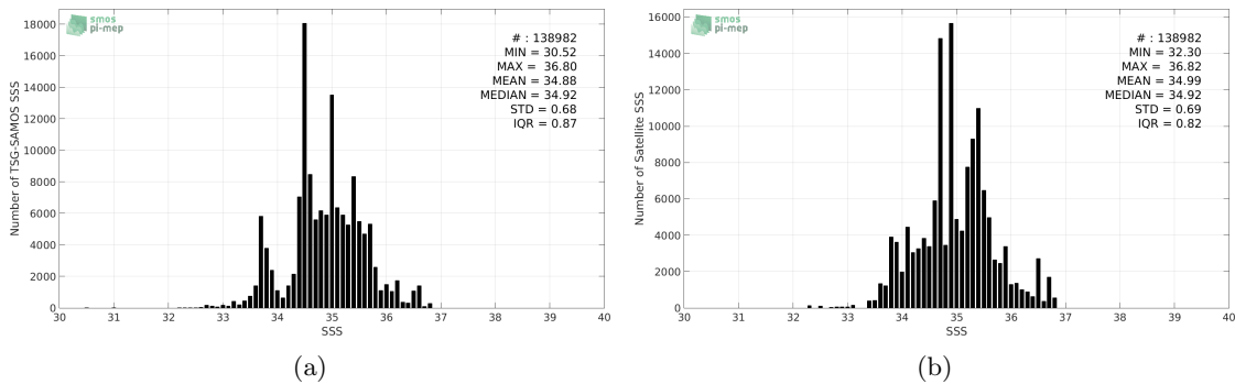
Figure 2: Histograms of SSS from TSG-SAMOS (a) and SMOS-L3-CATDS-CPDC-V3-MONTHLY-25KM (b) considering all match-up pairs per bins of 0.1 over the Indian Ocean Pi-MEP region and for the full satellite product period.
