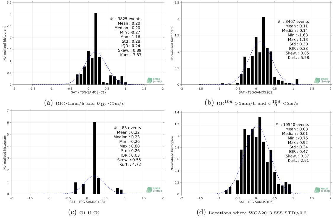
Figure 13: Normalized histogram of \Delta SSS (SMOS-L3-CATDS-CPDC-V3-MONTHLY-25KM - TSG-SAMOS) for 6 different subdatasets corresponding to: RR > 1\text{mm/h} and U_{10} < 5\text{m/s} (a), RR^{10d} > 5\text{mm/h} and U_{10}^{10d} < 5\text{m/s} (b), C1 U C2 (c), Locations where WOA2013 SSS STD > 0.2 (d).
