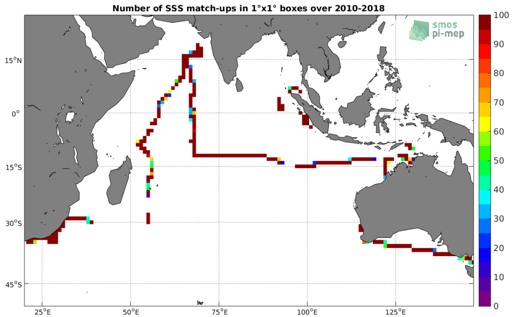
Figure 4: Number of SSS match-ups between TSG-SAMOS SSS and the SMOS-L3-CATDS-CPDC-V3-MONTHLY-25KM SSS product for the Indian Ocean Pi-MEP region over 1^\circ \times 1^\circ boxes and for the full satellite product period.
