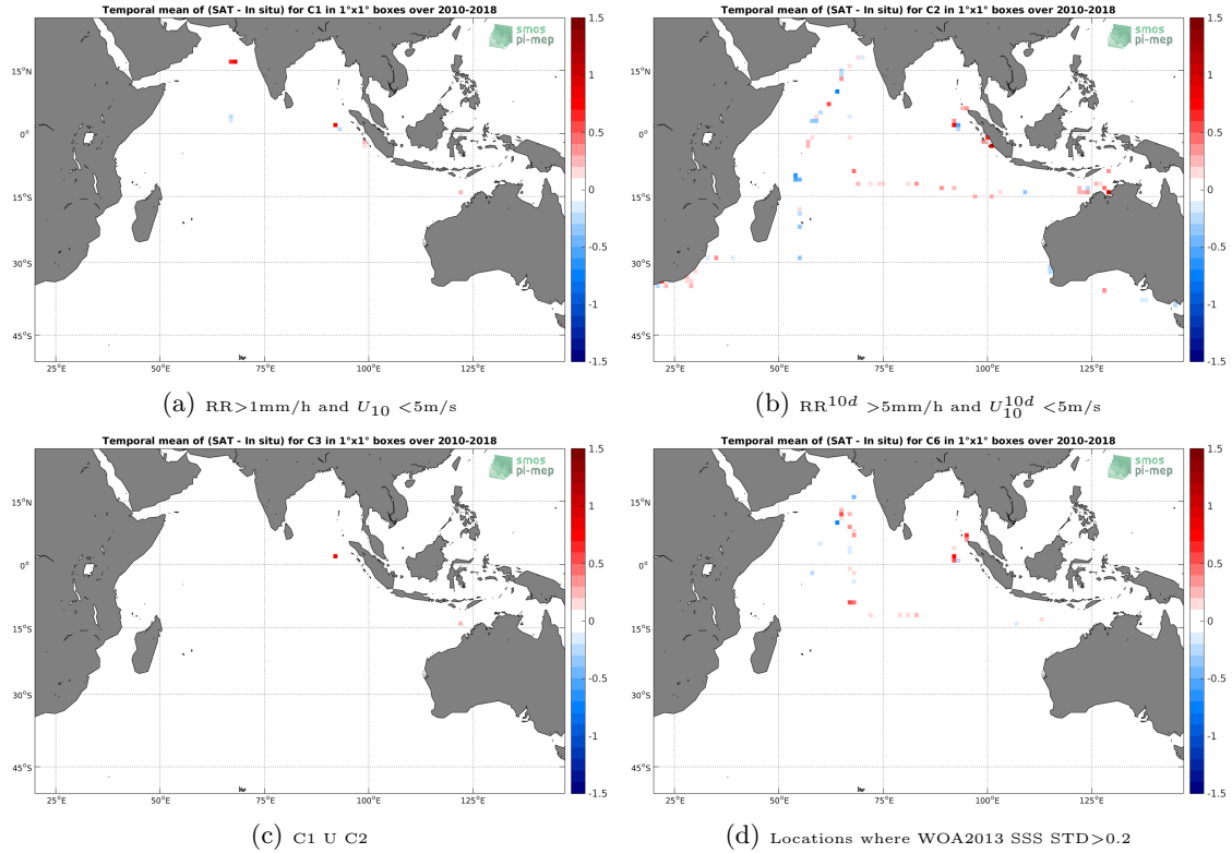
Figure 12: Temporal mean gridded over spatial boxes of size 1^\circ \times 1^\circ of \Delta SSS (SMOS-L3-CATDS-CPDC-V3-MONTHLY-25KM - TSG-SAMOS) for 4 different subdatasets corresponding to: RR > 1mm/h and U_{10} < 5\text{m/s} (a), RR^{10d} > 5\text{mm/h} and U_{10}^{10d} < 5\text{m/s} (b), C1 U C2 (c), Locations where WOA2013 SSS STD > 0.2 (d).
