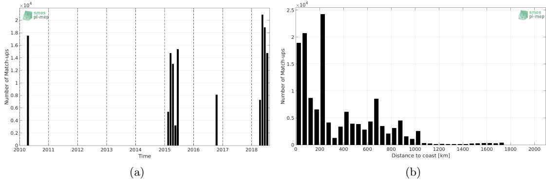
Figure 1: Number of match-ups between TSG-SAMOS and SMOS-L3-CATDS-CPDC-V3-MONTHLY-25KM SSS as a function of time (a) and as function of the distance to coast (b) over the Indian Ocean Pi-MEP region and for the full satellite product period.
