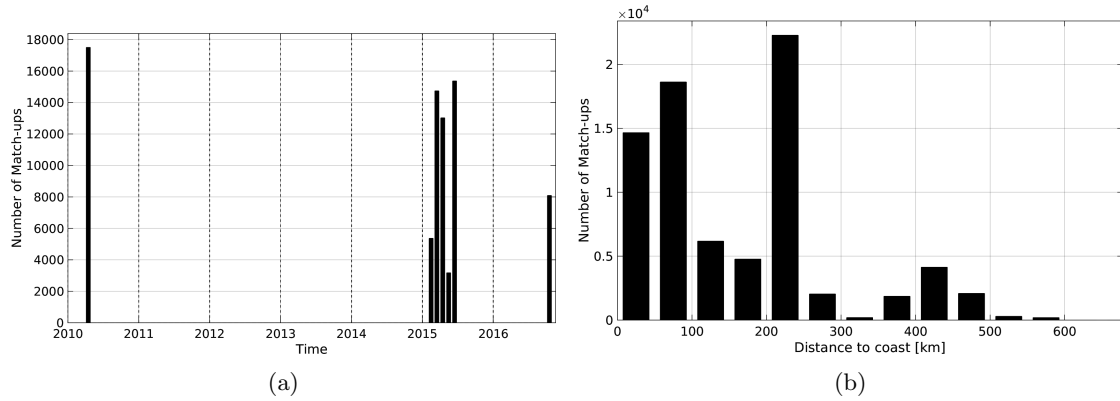
Figure 1: Number of match-ups between TSG-SAMOS and SMOS-L3-CATDS-CPDC-V3-MONTHLY-25KM SSS as a function of time (a) and as function of the distance to coast (b) over the Indian Ocean Pi-MEP region and for the full satellite product period.
