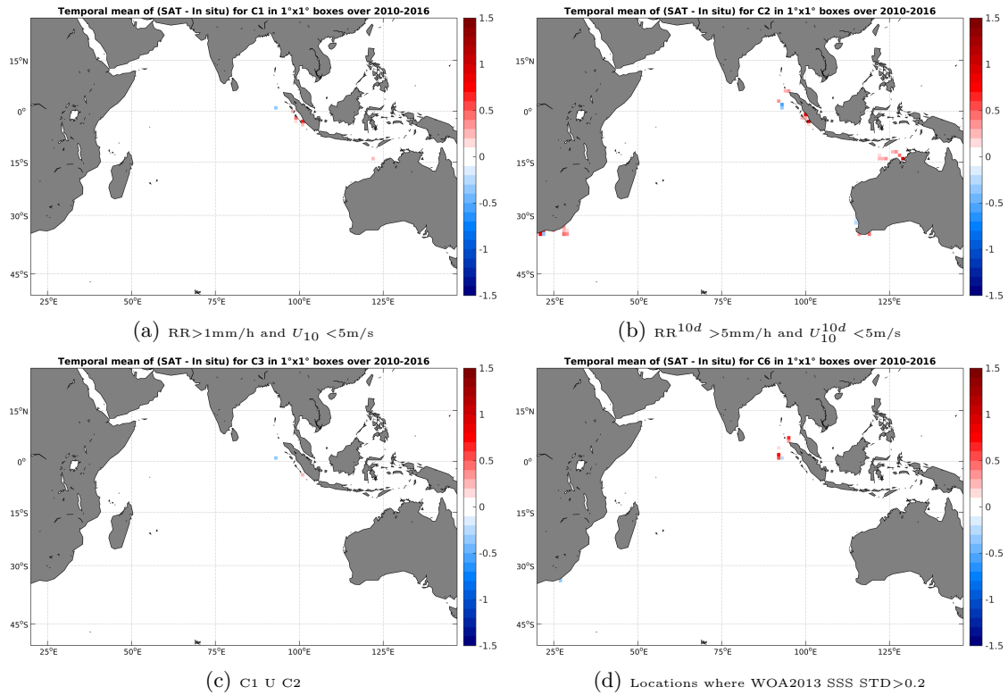
Figure 12: Temporal mean gridded over spatial boxes of size 1^\circ \times 1^\circ of \Delta SSS (SMOS-L3-CATDS-CPDC-V3-MONTHLY-25KM - TSG-SAMOS) for 4 different subdatasets corresponding to: RR > 1\text{mm/h} and U_{10} < 5\text{m/s} (a), RR^{10d} > 5\text{mm/h} and U_{10}^{10d} < 5\text{m/s} (b), C1 U C2 (c), Locations where WOA2013 SSS STD > 0.2 (d).
