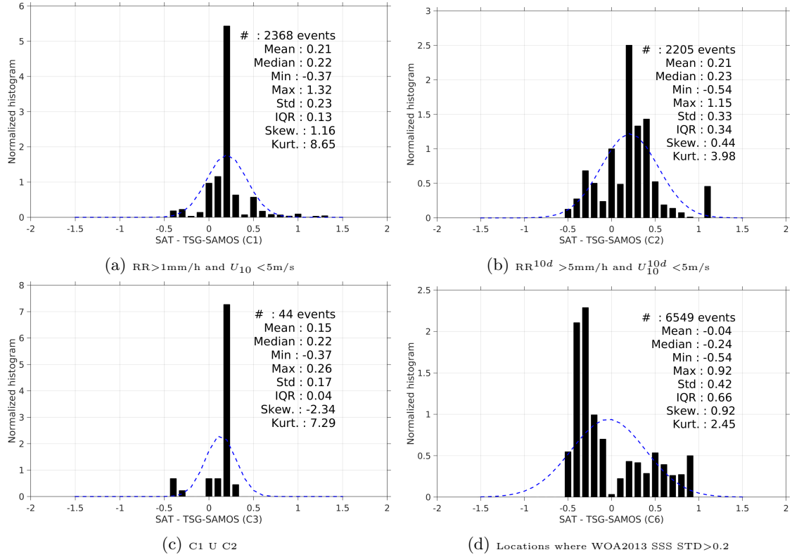
Figure 13: Normalized histogram of \Delta\text{SSS} (SMOS-L3-CATDS-CPDC-V3-MONTHLY-25KM - TSG-SAMOS) for 6 different subdatasets corresponding to: RR > 1mm/h and U_{10} < 5\text{m/s} (a), RR^{10d} > 5\text{mm/h} and U_{10}^{10d} < 5\text{m/s} (b), C1 U C2 (c), Locations where WOA2013 SSS STD > 0.2 (d).
