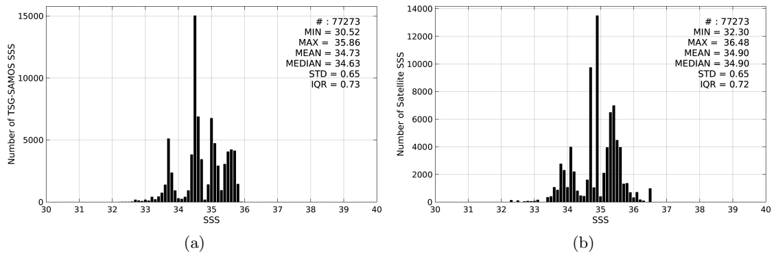
Figure 2: Histograms of SSS from TSG-SAMOS (a) and SMOS-L3-CATDS-CPDC-V3-MONTHLY-25KM (b) considering all match-up pairs per bins of 0.1 over the Indian Ocean Pi-MEP region and for the full satellite product period.
