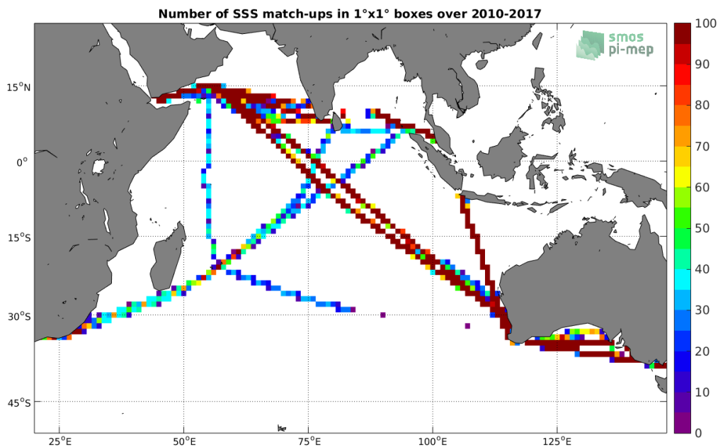
Figure 4: Number of SSS match-ups between TSG-LEGOS-DM SSS and the SMOS-L3-CATDS-CPDC-V3-MONTHLY-25KM SSS product for the Indian Ocean Pi-MEP region over 1^\circ \times 1^\circ boxes and for the full satellite product period.
