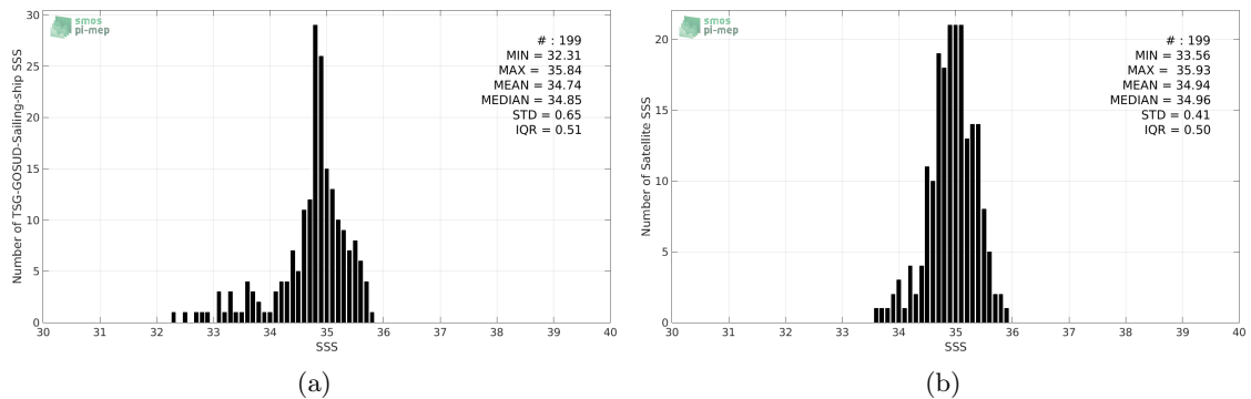
Figure 2: Histograms of SSS from TSG-GOSUD-Sailing-ship (a) and SMOS-L3-CATDS-CPDC-V3-MONTHLY-25KM (b) considering all match-up pairs per bins of 0.1 over the Indian Ocean Pi-MEP region and for the full satellite product period.
