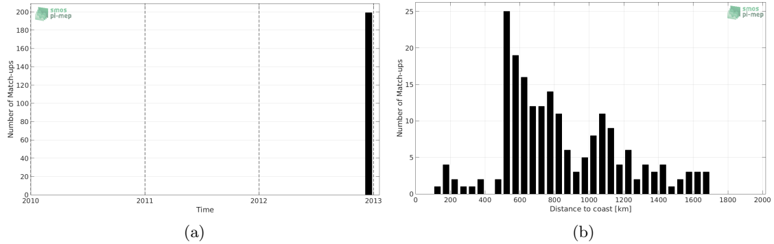
Figure 1: Number of match-ups between TSG-GOSUD-Sailing-ship and SMOS-L3-CATDS-CPDC-V3-MONTHLY-25KM SSS as a function of time (a) and as function of the distance to coast (b) over the Indian Ocean Pi-MEP region and for the full satellite product period.
