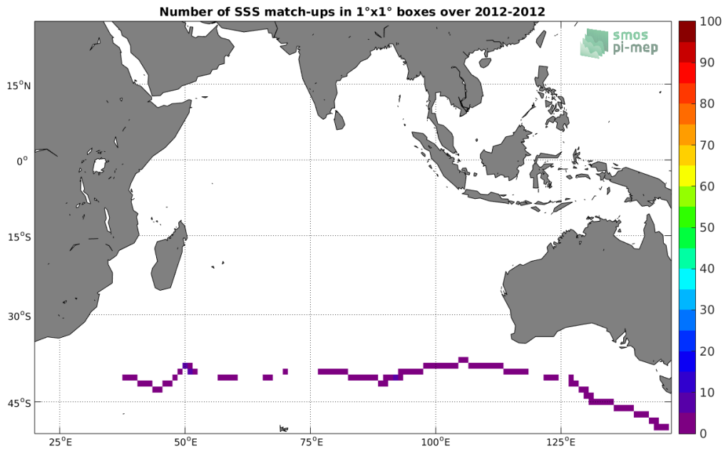
Figure 4: Number of SSS match-ups between TSG-GOSUD-Sailing-ship SSS and the SMOS-L3-CATDS-CPDC-V3-MONTHLY-25KM SSS product for the Indian Ocean Pi-MEP region over 1^\circ \times 1^\circ boxes and for the full satellite product period.
