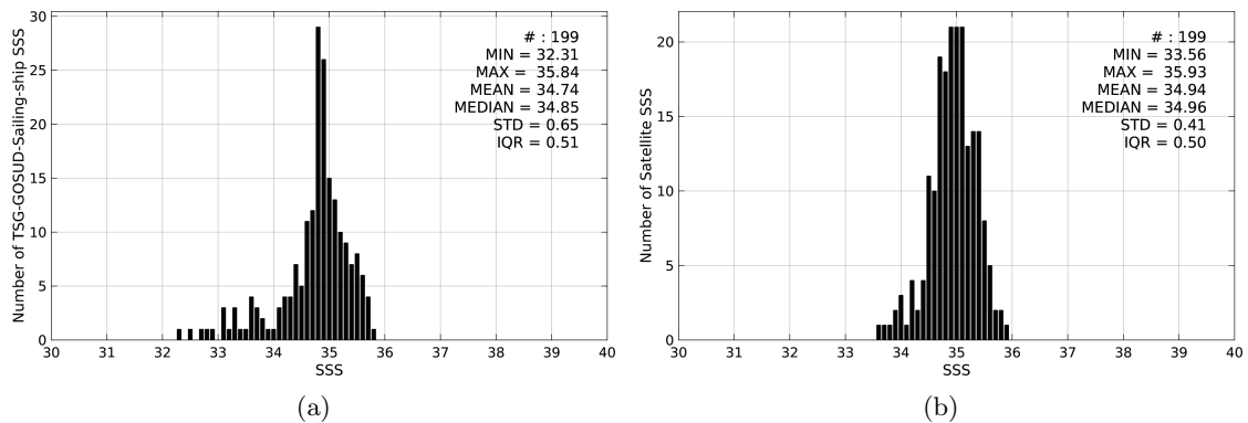
Figure 2: Histograms of SSS from TSG-GOSUD-Sailing-ship (a) and SMOS-L3-CATDS-CPDC-V3-MONTHLY-25KM (b) considering all match-up pairs per bins of 0.1 over the Indian Ocean Pi-MEP region and for the full satellite product period.
