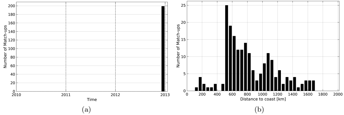
Figure 1: Number of match-ups between TSG-GOSUD-Sailing-ship and SMOS-L3-CATDS-CPDC-V3-MONTHLY-25KM SSS as a function of time (a) and as function of the distance to coast (b) over the Indian Ocean Pi-MEP region and for the full satellite product period.
