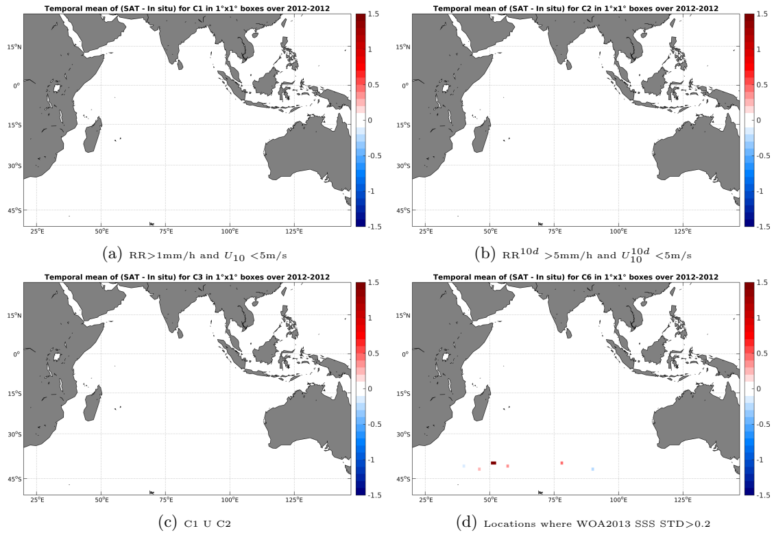
Figure 12: Temporal mean gridded over spatial boxes of size 1°x1° of \Delta SSS (SMOS-L3-CATDS-CPDC-V3-MONTHLY-25KM - TSG-GOSUD-Sailing-ship) for 4 different subdatasets corresponding to:RR>1mm/h and U_{10} < 5m/s (a), RR^{10d} > 5mm/h and U_{10}^{10d} < 5m/s (b), C1 U C2 (c),Locations where WOA2013 SSS STD>0.2 (d).
