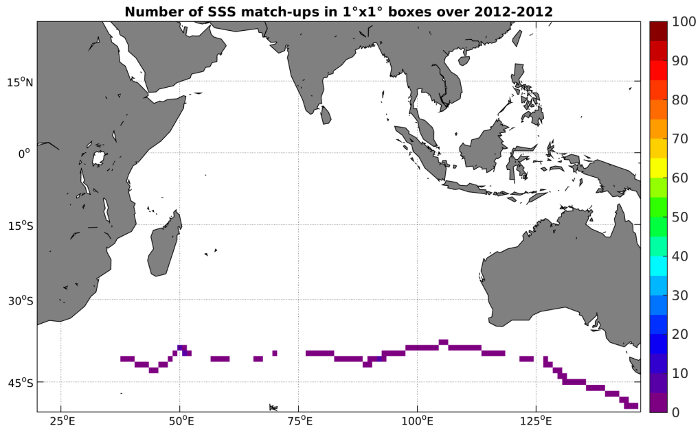
Figure 4: Number of SSS match-ups between TSG-GOSUD-Sailing-ship SSS and the SMOS-L3-CATDS-CPDC-V3-MONTHLY-25KM SSS product for the Indian Ocean Pi-MEP region over 1^{\circ} \times 1^{\circ} boxes and for the full satellite product period.
