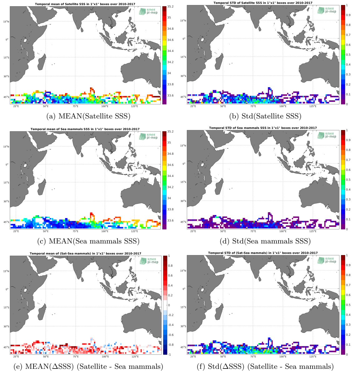
Figure 6: Temporal mean (left) and Std (right) of SSS from SMOS-L3-CATDS-CPDC-V3-MONTHLY-25KM (top), Sea mammals (middle), and of \Delta SSS (Satellite - Sea mammals). Only match-up pairs are used to generate these maps.
