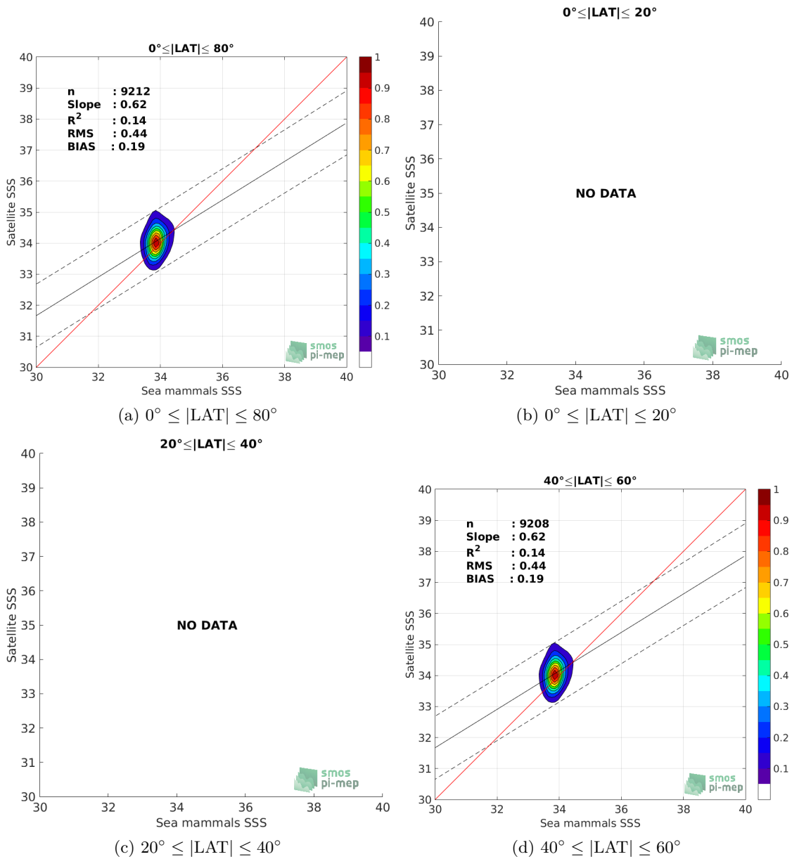
Figure 9: Contour maps of the concentration of SMOS-L3-CATDS-CPDC-V3-MONTHLY-25KM SSS (y-axis) versus Sea mammals SSS (x-axis) at match-up pairs for different latitude bands. For each plot, the red line shows x=y . The black thin and dashed lines indicate a linear fit through the data cloud and the \pm 95\% confidence levels, respectively. The number match-up pairs n , the slope and R^2 coefficient of the linear fit, the root mean square (RMS) and the mean bias between satellite and in situ data are indicated for each latitude band in each plots.
