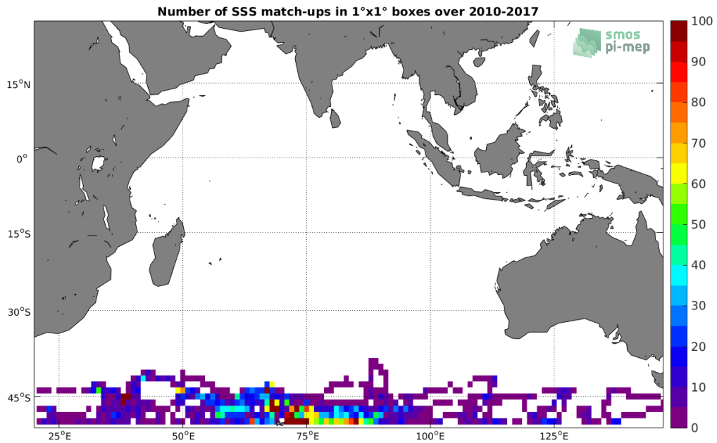
Figure 4: Number of SSS match-ups between Sea mammals SSS and the SMOS-L3-CATDS-CPDC-V3-MONTHLY-25KM SSS product for the Indian Ocean Pi-MEP region over 1^{\circ} \times 1^{\circ} boxes and for the full satellite product period.
