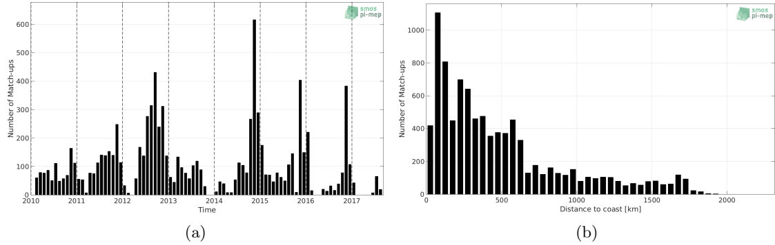
Figure 1: Number of match-ups between Sea mammals and SMOS-L3-CATDS-CPDC-V3-MONTHLY-25KM SSS as a function of time (a) and as function of the distance to coast (b) over the Indian Ocean Pi-MEP region and for the full satellite product period.
