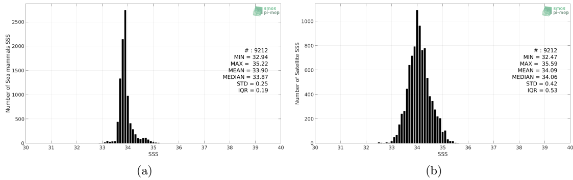
Figure 2: Histograms of SSS from Sea mammals (a) and SMOS-L3-CATDS-CPDC-V3-MONTHLY-25KM (b) considering all match-up pairs per bins of 0.1 over the Indian Ocean Pi-MEP region and for the full satellite product period.
