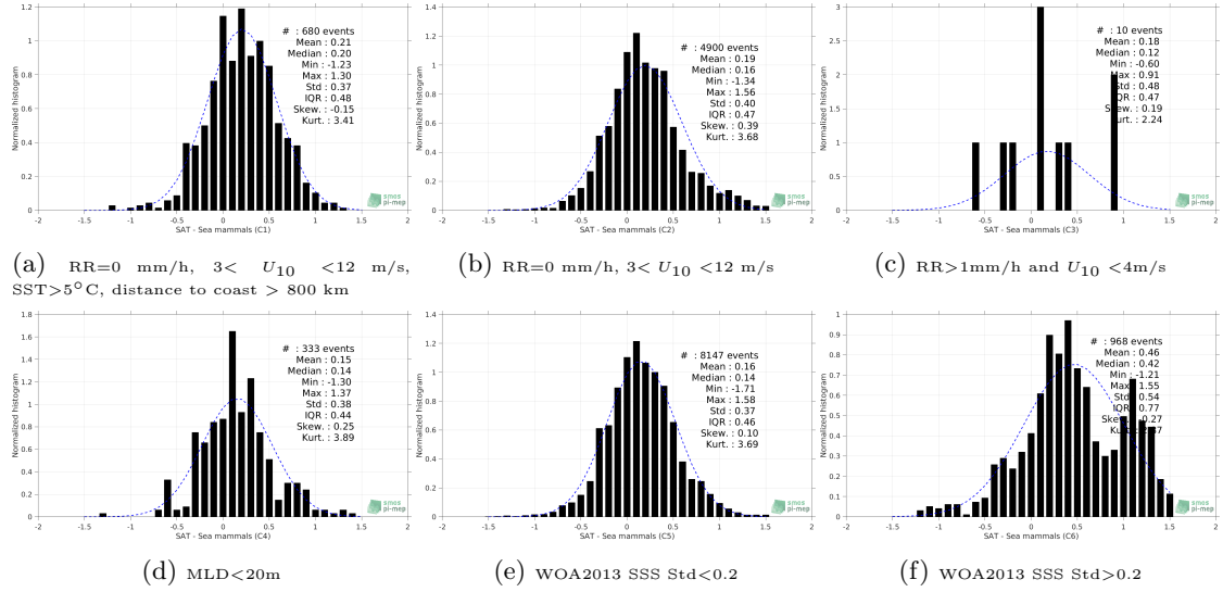
Figure 13: Normalized histogram of \Delta SSS (SMOS-L3-CATDS-CPDC-V3-MONTHLY-25KM - Sea mammals) for 6 different subdatasets corresponding to: RR=0 mm/h, 3 < U_{10} < 12 m/s, SST>5°C, distance to coast > 800 km (a), RR=0 mm/h, 3 < U_{10} < 12 m/s (b), RR>1mm/h and U_{10} < 4 m/s (c), MLD<20m (d), WOA2013 SSS Std<0.2 (e), WOA2013 SSS Std>0.2 (f).
