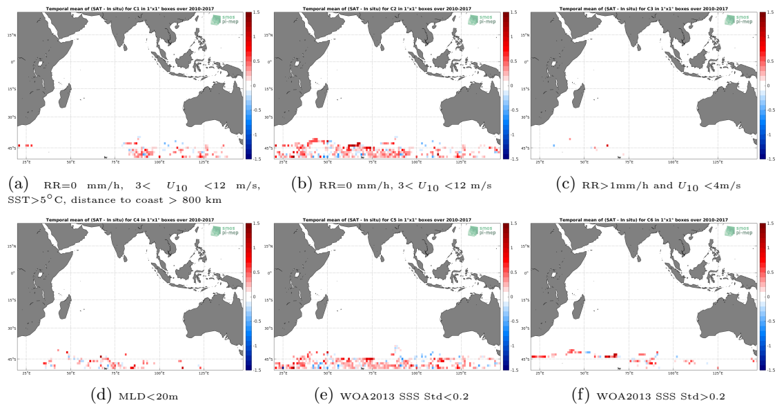
Figure 12: Temporal mean gridded over spatial boxes of size 1^\circ \times 1^\circ of \Delta SSS (SMOS-L3-CATDS-CPDC-V3-MONTHLY-25KM - Sea mammals) for 6 different subdatasets corresponding to:RR=0 mm/h, 3 < U_{10} < 12 m/s, SST >5^\circ C, distance to coast > 800 km (a), RR=0 mm/h, 3 < U_{10} < 12 m/s (b), RR >1 mm/h and U_{10} < 4 m/s (c),MLD <20 m (d),WOA2013 SSS Std <0.2 (e),WOA2013 SSS Std >0.2 (f).
