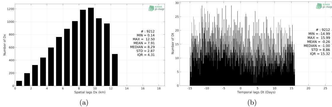
Figure 5: Histograms of the spatial (a) and temporal (b) lags between the time of the Sea mammals measurements and the date of the corresponding SMOS-L3-CATDS-CPDC-V3-MONTHLY-25KM SSS product.
