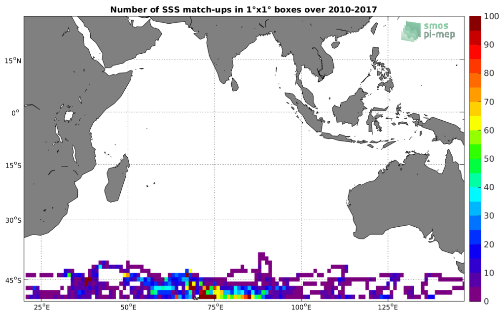
Figure 4: Number of SSS match-ups between Sea mammals SSS and the SMOS-L3-CATDS-CPDC-V3-MONTHLY-25KM SSS product for the Indian Ocean Pi-MEP region over 1^\circ \times 1^\circ boxes and for the full satellite product period.
