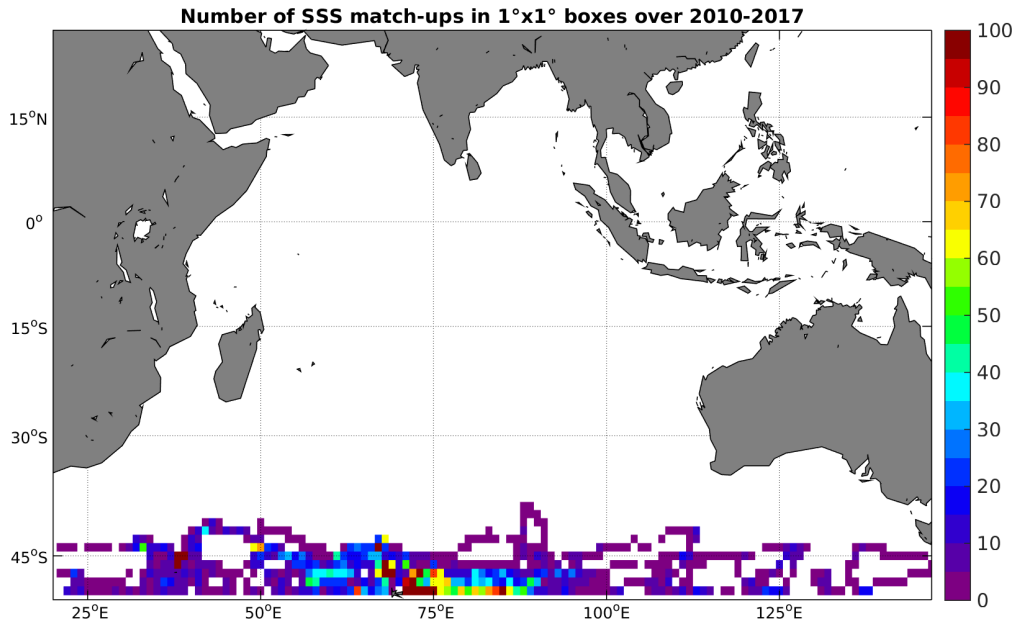
Figure 4: Number of SSS match-ups between Sea mammals SSS and the SMOS-L3-CATDS-CPDC-V3-MONTHLY-25KM SSS product for the Indian Ocean Pi-MEP region over 1°x1° boxes and for the full satellite product period.
