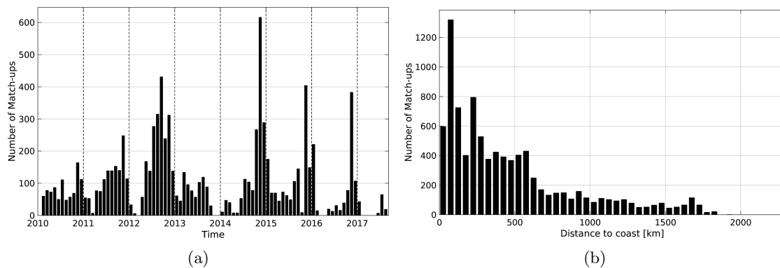
Figure 1: Number of match-ups between Sea mammals and SMOS-L3-CATDS-CPDC-V3-MONTHLY-25KM SSS as a function of time (a) and as function of the distance to coast (b) over the Indian Ocean Pi-MEP region and for the full satellite product period.
