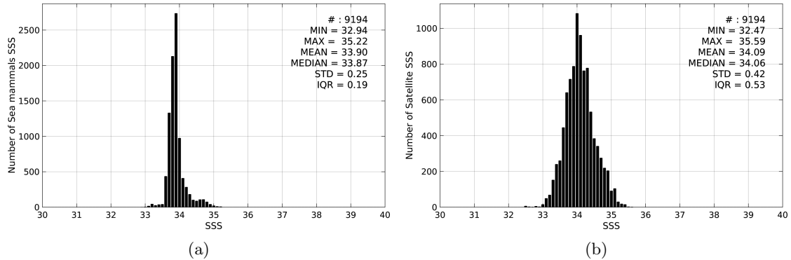
Figure 2: Histograms of SSS from Sea mammals (a) and SMOS-L3-CATDS-CPDC-V3-MONTHLY-25KM (b) considering all match-up pairs per bins of 0.1 over the Indian Ocean Pi-MEP region and for the full satellite product period.
