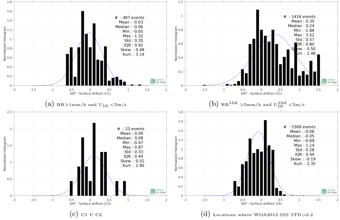
Figure 12: Normalized histogram of \Delta SSS (SMOS-L3-CATDS-CPDC-V3-MONTHLY-25KM - Surface drifters) for 6 different subdatasets corresponding to: RR > 1\text{mm/h} and U_{10} < 5\text{m/s} (a), RR^{10d} > 5\text{mm/h} and U_{10}^{10d} < 5\text{m/s} (b), C1 U C2 (c), Locations where WOA2013 SSS STD > 0.2 (d).
