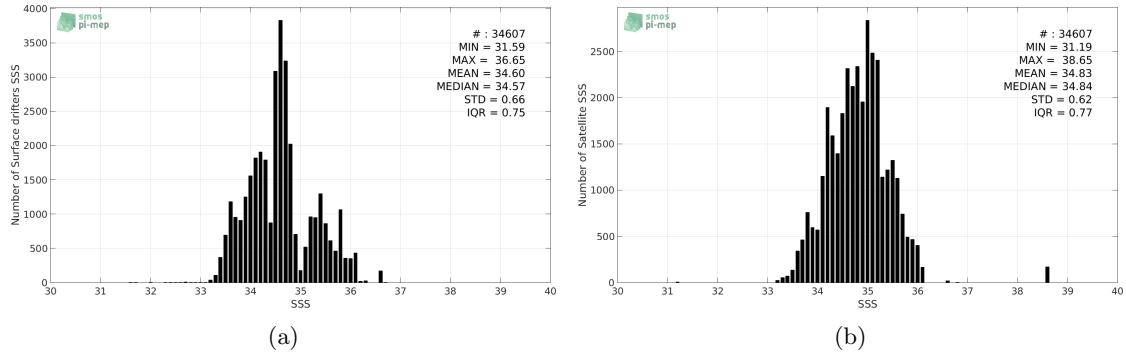
Figure 2: Histograms of SSS from Surface drifters (a) and SMOS-L3-CATDS-CPDC-V3-MONTHLY-25KM (b) considering all match-up pairs per bins of 0.1 over the Indian Ocean Pi-MEP region and for the full satellite product period.
