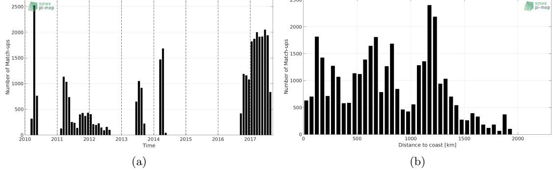
Figure 1: Number of match-ups between Surface drifters and SMOS-L3-CATDS-CPDC-V3-MONTHLY-25KM SSS as a function of time (a) and as function of the distance to coast (b) over the Indian Ocean Pi-MEP region and for the full satellite product period.
