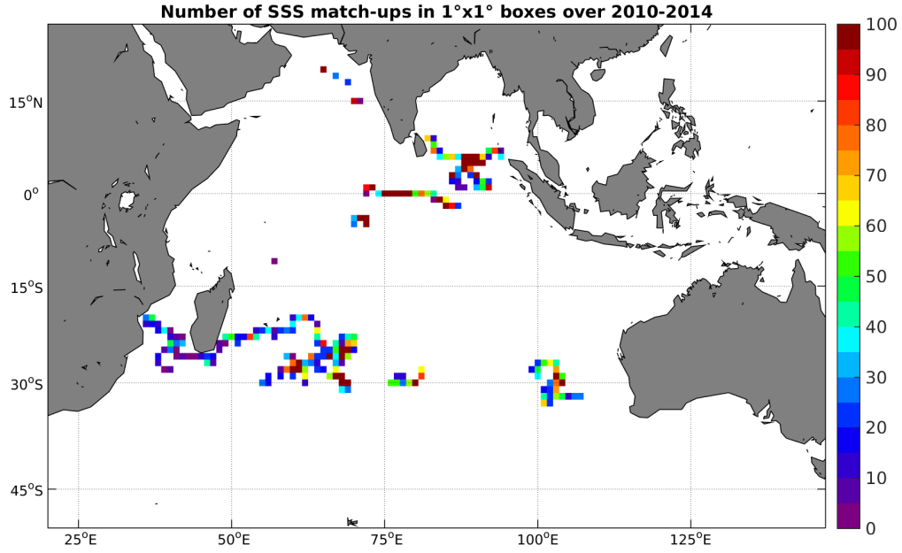
Figure 3: Number of SSS match-ups between Surface drifters SSS and the SMOS-L3-CATDS-CPDC-V3-MONTHLY-25KM SSS product for the Indian Ocean Pi-MEP region over 1^\circ \times 1^\circ boxes and for the full satellite product period.
