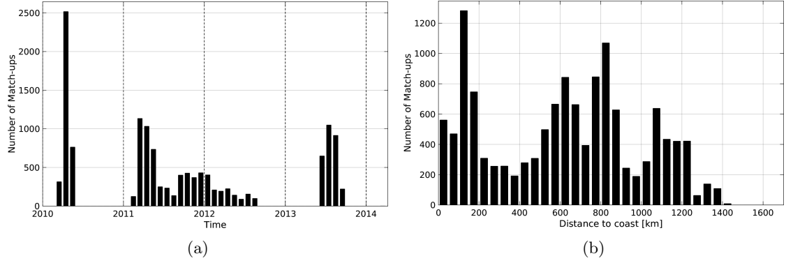
Figure 1: Number of match-ups between Surface drifters and SMOS-L3-CATDS-CPDC-V3-MONTHLY-25KM SSS as a function of time (a) and as function of the distance to coast (b) over the Indian Ocean Pi-MEP region and for the full satellite product period.
