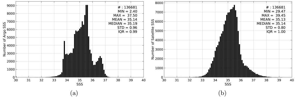
Figure 2: Histograms of SSS from Argo (a) and SMOS-L3-CATDS-CPDC-V3-MONTHLY-25KM (b) considering all match-up pairs per bins of 0.1 over the Indian Ocean Pi-MEP region and for the full satellite product period.
