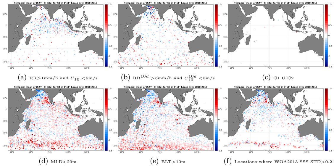
Figure 12: Temporal mean gridded over spatial boxes of size 1^\circ \times 1^\circ of \Delta SSS (SMOS-L3-CATDS-CPDC-V3-MONTHLY-25KM - Argo) for 6 different subdatasets corresponding to:RR>1mm/h and U_{10} < 5m/s (a), RR^{10d} > 5mm/h and U_{10}^{10d} < 5m/s (b), C1 U C2 (c),MLD<20m (d),BLT>10m (e),Locations where WOA2013 SSS STD>0.2 (f).
