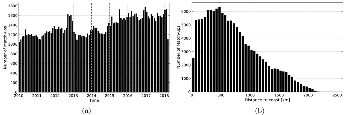
Figure 1: Number of match-ups between Argo and SMOS-L3-CATDS-CPDC-V3-MONTHLY-25KM SSS as a function of time (a) and as function of the distance to coast (b) over the Indian Ocean Pi-MEP region and for the full satellite product period.
