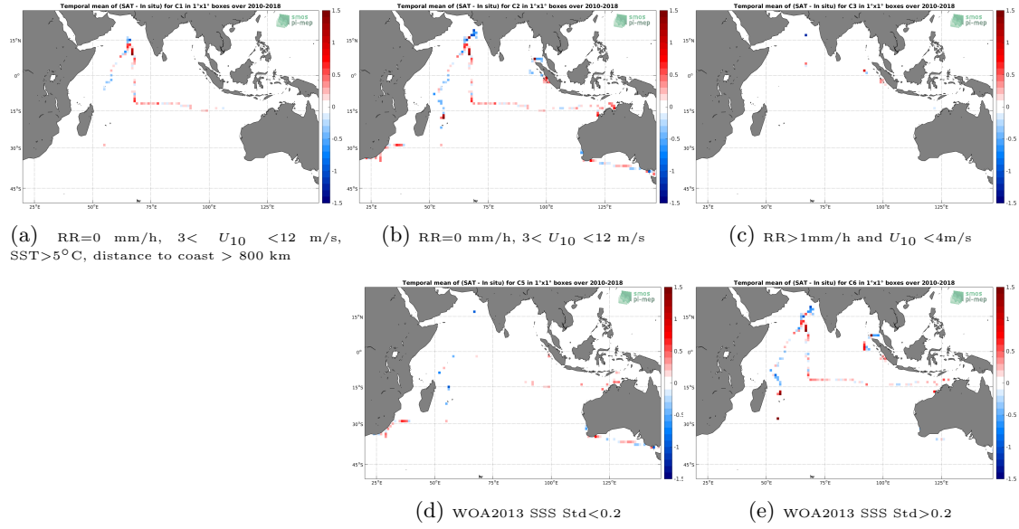
Figure 12: Temporal mean gridded over spatial boxes of size 1^\circ \times 1^\circ of \Delta SSS (SMOS-L3-CATDS-CPDC-V3-10DAYS-25KM - TSG-SAMOS) for 5 different subdatasets corresponding to: RR=0 mm/h, 3 < U_{10} < 12 m/s, SST >5^\circ C, distance to coast > 800 km (a), RR=0 mm/h, 3 < U_{10} < 12 m/s (b), RR >1 mm/h and U_{10} < 4 m/s (c), WOA2013 SSS Std <0.2 (d), WOA2013 SSS Std >0.2 (e).
