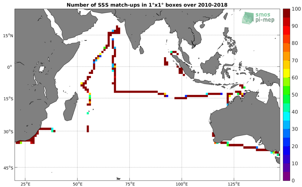
Figure 4: Number of SSS match-ups between TSG-SAMOS SSS and the SMOS-L3-CATDS-CPDC-V3-10DAYS-25KM SSS product for the Indian Ocean Pi-MEP region over 1^\circ \times 1^\circ boxes and for the full satellite product period.
