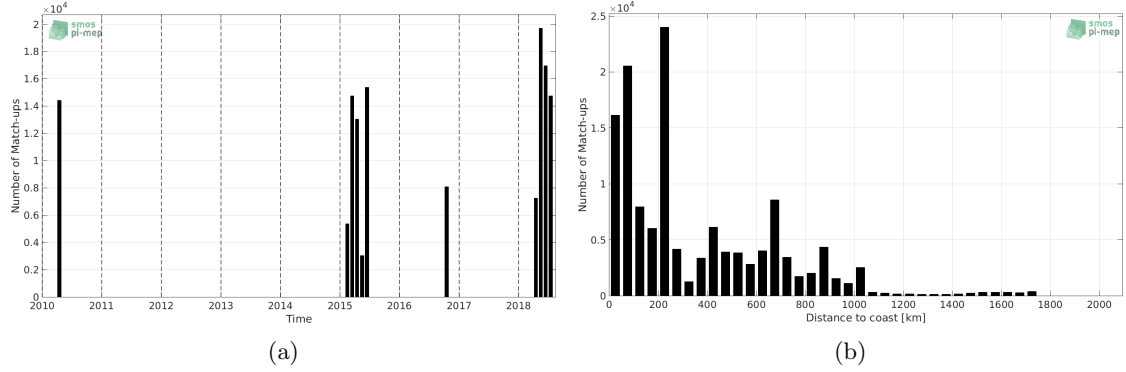
Figure 1: Number of match-ups between TSG-SAMOS and SMOS-L3-CATDS-CPDC-V3-10DAYS-25KM SSS as a function of time (a) and as function of the distance to coast (b) over the Indian Ocean Pi-MEP region and for the full satellite product period.
