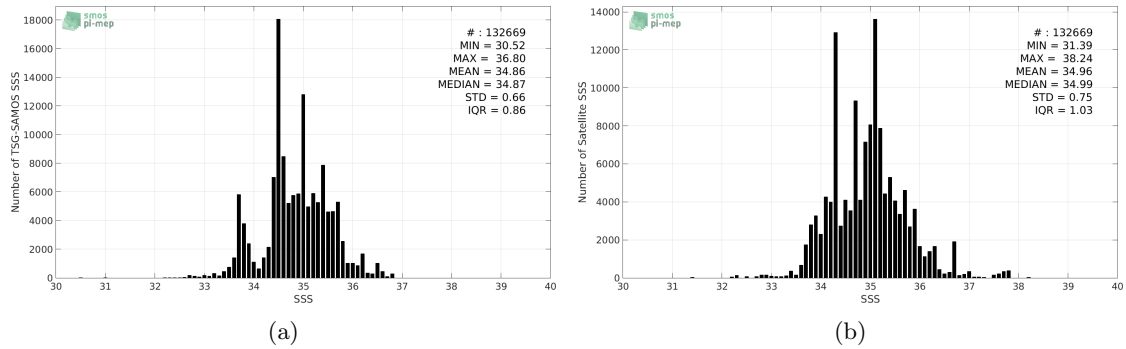
Figure 2: Histograms of SSS from TSG-SAMOS (a) and SMOS-L3-CATDS-CPDC-V3-10DAYS-25KM (b) considering all match-up pairs per bins of 0.1 over the Indian Ocean Pi-MEP region and for the full satellite product period.
