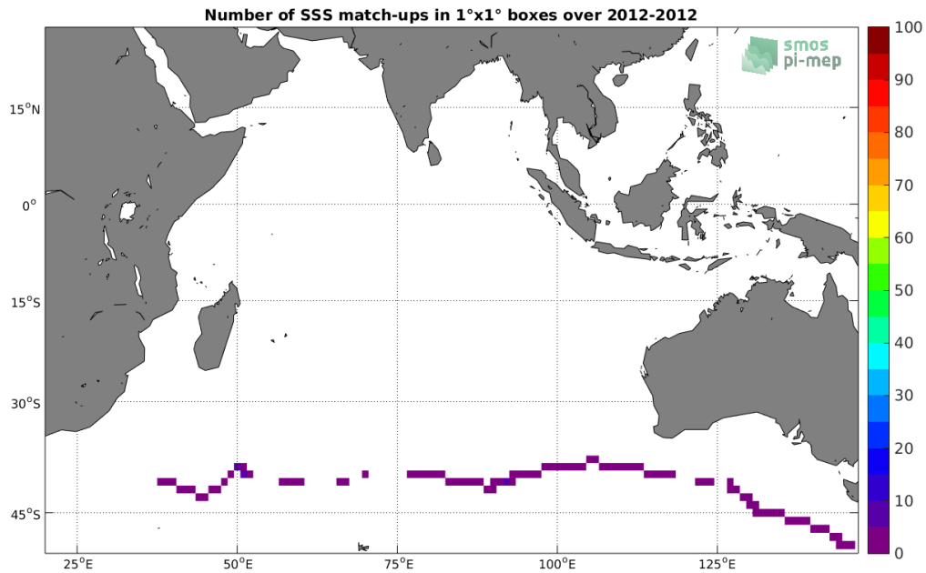
Figure 4: Number of SSS match-ups between TSG-GOSUD-Sailing-ship SSS and the SMOS-L3-CATDS-CPDC-V3-10DAYS-25KM SSS product for the Indian Ocean Pi-MEP region over 1^\circ \times 1^\circ boxes and for the full satellite product period.
