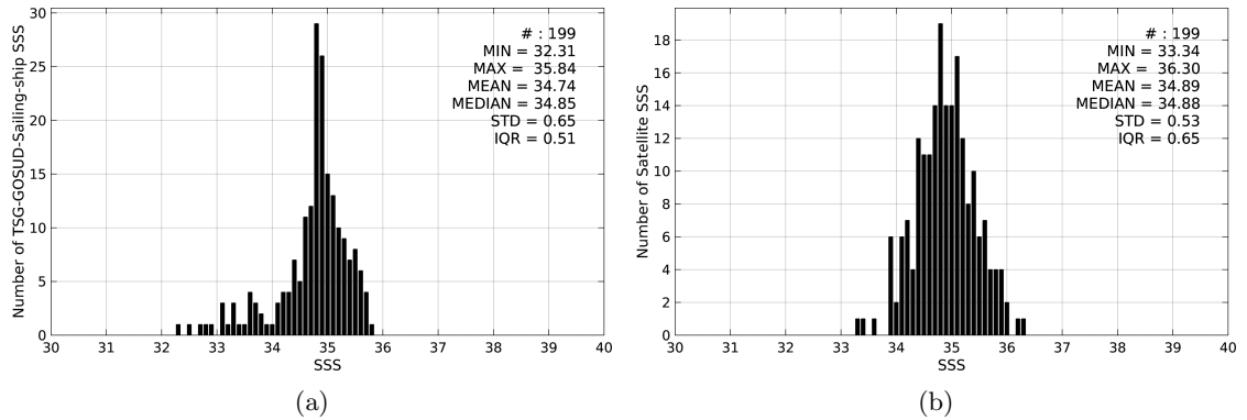
Figure 2: Histograms of SSS from TSG-GOSUD-Sailing-ship (a) and SMOS-L3-CATDS-CPDC-V3-10DAYS-25KM (b) considering all match-up pairs per bins of 0.1 over the Indian Ocean Pi-MEP region and for the full satellite product period.
