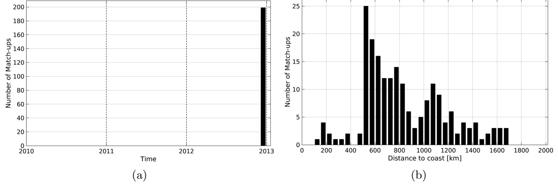
Figure 1: Number of match-ups between TSG-GOSUD-Sailing-ship and SMOS-L3-CATDS-CPDC-V3-10DAYS-25KM SSS as a function of time (a) and as function of the distance to coast (b) over the Indian Ocean Pi-MEP region and for the full satellite product period.
