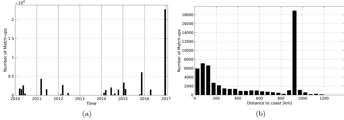
Figure 1: Number of match-ups between TSG-GOSUD-Research-vessel and SMOS-L3-CATDS-CPDC-V3-10DAYS-25KM SSS as a function of time (a) and as function of the distance to coast (b) over the Indian Ocean Pi-MEP region and for the full satellite product period.
