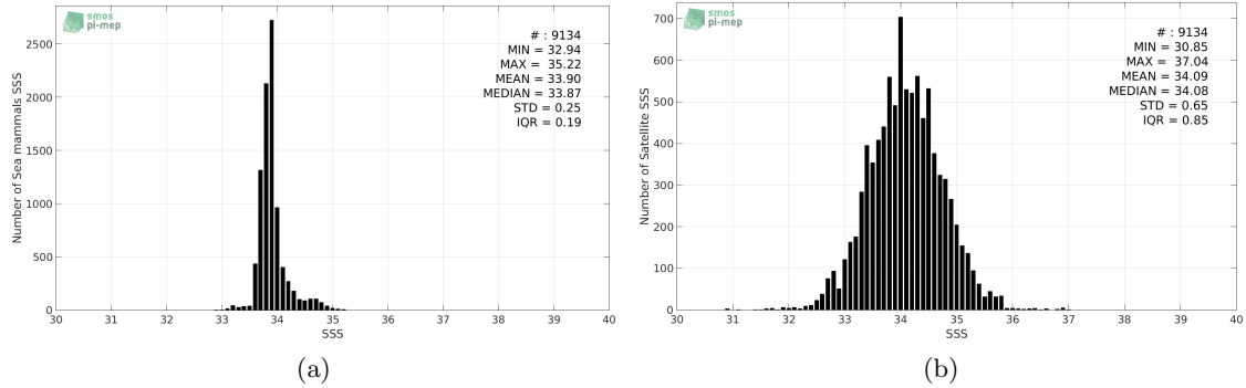
Figure 2: Histograms of SSS from Sea mammals (a) and SMOS-L3-CATDS-CPDC-V3-10DAYS-25KM (b) considering all match-up pairs per bins of 0.1 over the Indian Ocean Pi-MEP region and for the full satellite product period.
