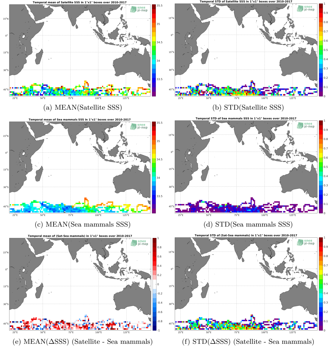
Figure 6: Temporal mean (left) and STD (right) of SSS from SMOS-L3-CATDS-CPDC-V3-10DAYS-25KM (top), Sea mammals (middle), and of \Delta SSS (Satellite - Sea mammals). Only match-up pairs are used to generate these maps.
