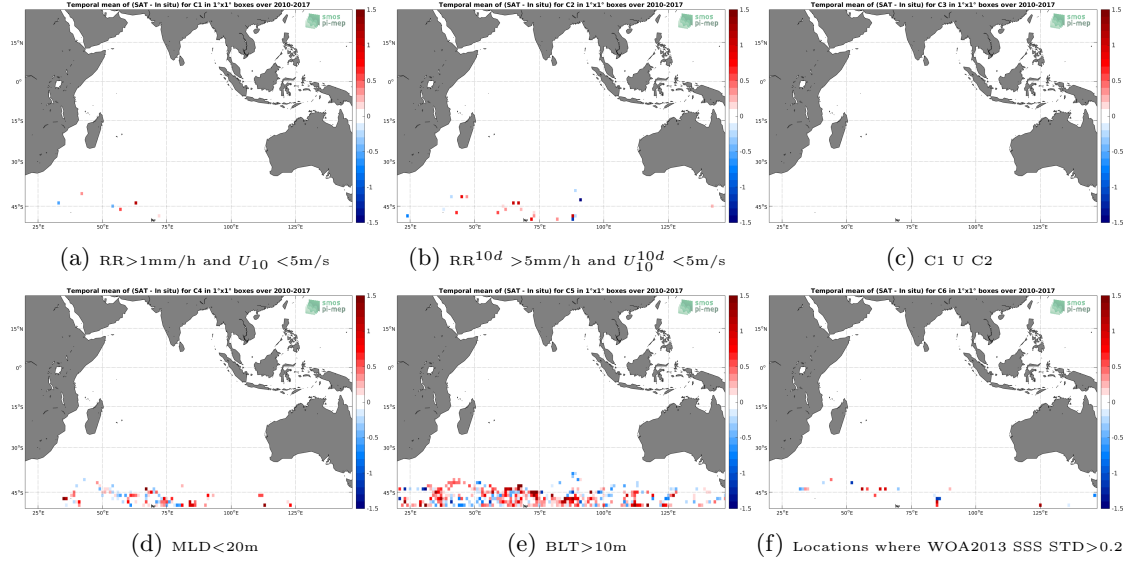
Figure 12: Temporal mean gridded over spatial boxes of size 1^\circ \times 1^\circ of \Delta\text{SSS} (SMOS-L3-CATDS-CPDC-V3-10DAYS-25KM - Sea mammals) for 6 different subdatasets corresponding to: \text{RR} > 1\text{mm/h} and U_{10} < 5\text{m/s} (a), \text{RR}^{10d} > 5\text{mm/h} and U_{10}^{10d} < 5\text{m/s} (b), C1 U C2 (c), \text{MLD} < 20\text{m} (d), \text{BLT} > 10\text{m} (e), Locations where WOA2013 SSS STD > 0.2 (f).
