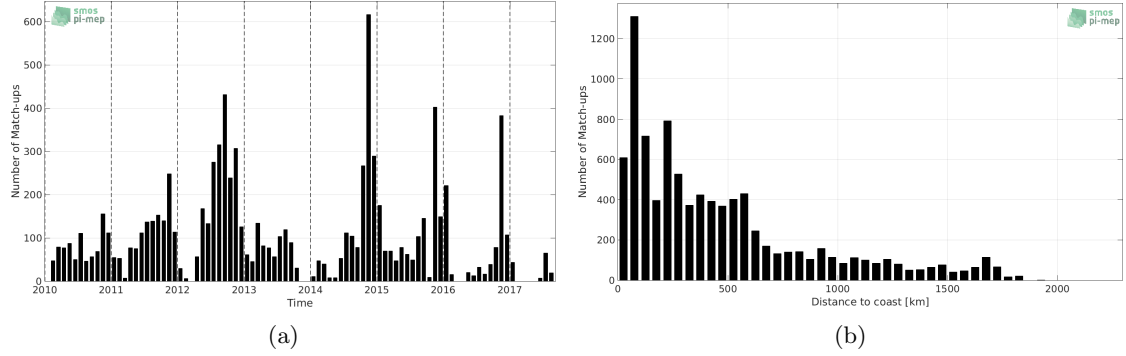
Figure 1: Number of match-ups between Sea mammals and SMOS-L3-CATDS-CPDC-V3-10DAYS-25KM SSS as a function of time (a) and as function of the distance to coast (b) over the Indian Ocean Pi-MEP region and for the full satellite product period.
