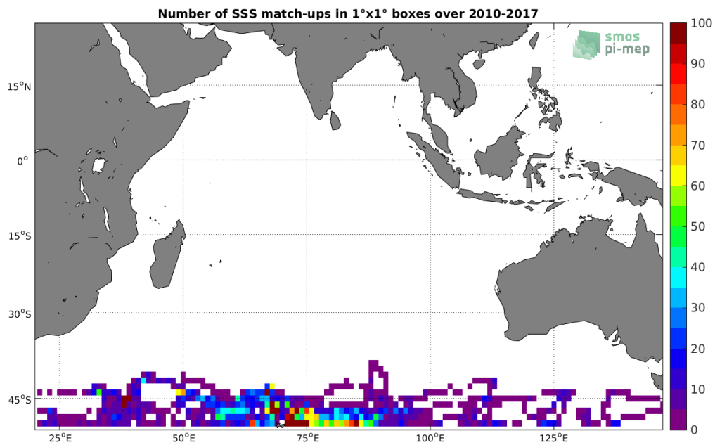
Figure 4: Number of SSS match-ups between Sea mammals SSS and the SMOS-L3-CATDS-CPDC-V3-10DAYS-25KM SSS product for the Indian Ocean Pi-MEP region over 1^\circ \times 1^\circ boxes and for the full satellite product period.
