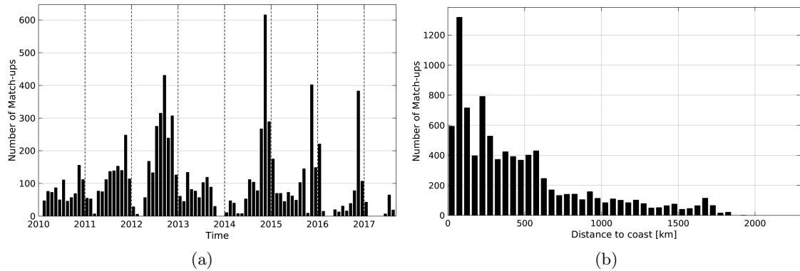
Figure 1: Number of match-ups between Sea mammals and SMOS-L3-CATDS-CPDC-V3-10DAYS-25KM SSS as a function of time (a) and as function of the distance to coast (b) over the Indian Ocean Pi-MEP region and for the full satellite product period.
