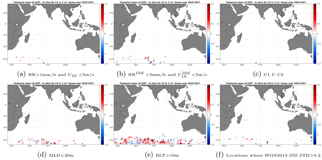
Figure 12: Temporal mean gridded over spatial boxes of size 1^\circ \times 1^\circ of \Delta SSS (SMOS-L3-CATDS-CPDC-V3-10DAYS-25KM - Sea mammals) for 6 different subdatasets corresponding to: RR > 1\text{mm/h} and U_{10} < 5\text{m/s} (a), RR^{10d} > 5\text{mm/h} and U_{10}^{10d} < 5\text{m/s} (b), C1 U C2 (c), MLD < 20\text{m} (d), BLT > 10\text{m} (e), Locations where WOA2013 SSS STD > 0.2 (f).
