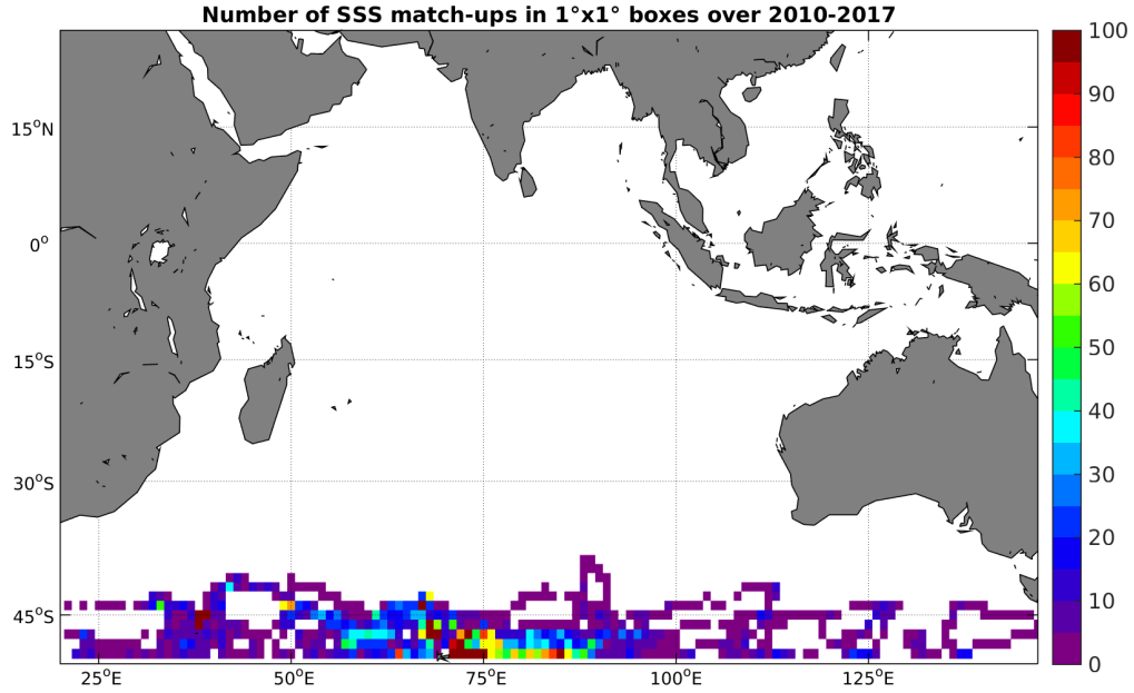
Figure 4: Number of SSS match-ups between Sea mammals SSS and the SMOS-L3-CATDS-CPDC-V3-10DAYS-25KM SSS product for the Indian Ocean Pi-MEP region over 1^\circ \times 1^\circ boxes and for the full satellite product period.
