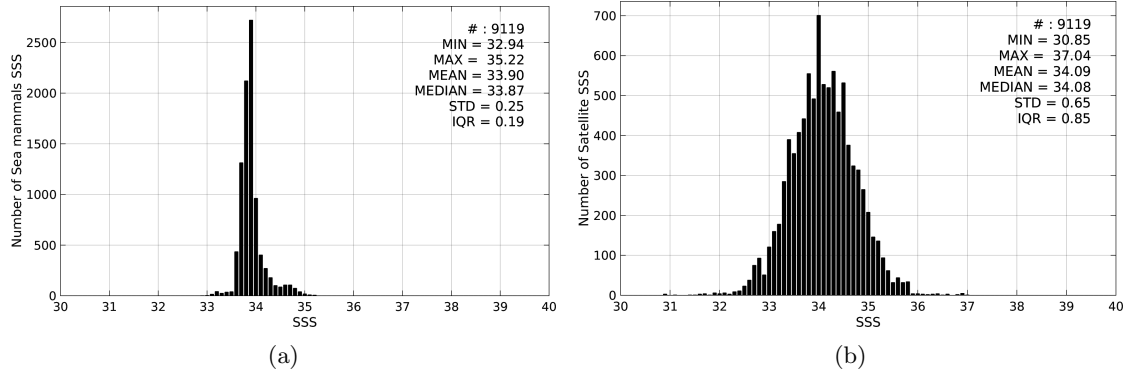
Figure 2: Histograms of SSS from Sea mammals (a) and SMOS-L3-CATDS-CPDC-V3-10DAYS-25KM (b) considering all match-up pairs per bins of 0.1 over the Indian Ocean Pi-MEP region and for the full satellite product period.
