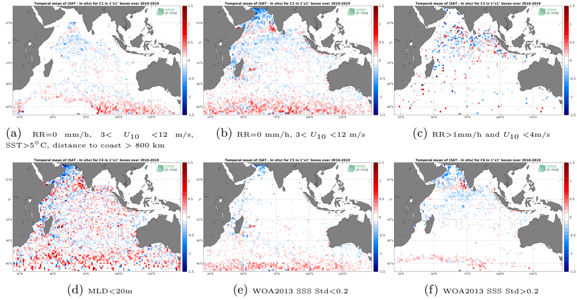
Figure 12: Temporal mean gridded over spatial boxes of size 1^\circ \times 1^\circ of \Delta SSS (SMOS-L3-CATDS-CPDC-V3-10DAYS-25KM - Argo) for 6 different subdatasets corresponding to: RR=0 mm/h, 3 < U_{10} < 12 m/s, SST > 5^\circ C , distance to coast > 800 km (a), RR=0 mm/h, 3 < U_{10} < 12 m/s (b), RR > 1 mm/h and U_{10} < 4 m/s (c), MLD < 20 m (d), WOA2013 SSS Std < 0.2 (e), WOA2013 SSS Std > 0.2 (f).
