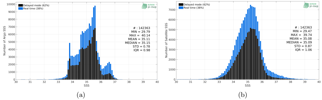
Figure 2: Histograms of SSS from Argo (a) and SMOS-L3-CATDS-CPDC-V3-10DAYS-25KM (b) considering all match-up pairs per bins of 0.1 over the Indian Ocean Pi-MEP region and for the full satellite product period.
