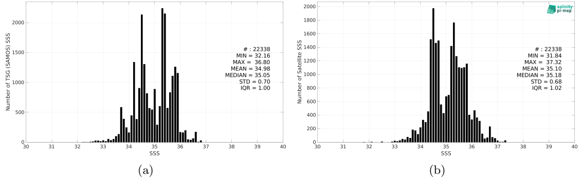
Figure 2: Histograms of SSS from TSG (SAMOS) (a) and SMOS SSS L3 v2 - 9-Days (BEC) (b) considering all match-up pairs per bins of 0.1 over the Indian Ocean Pi-MEP region and for the full satellite product period.
