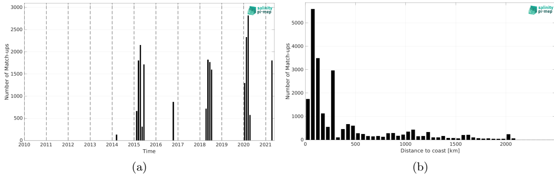
Figure 1: Number of match-ups between TSG (SAMOS) and SMOS SSS L3 v2 - 9-Days (BEC) SSS as a function of time (a) and as function of the distance to coast (b) over the Indian Ocean Pi-MEP region and for the full satellite product period.
