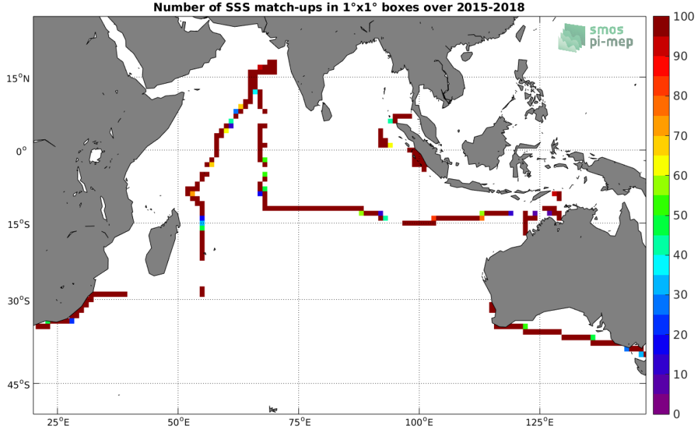
Figure 4: Number of SSS match-ups between TSG (SAMOS) SSS and the SMOS SSS L3 v2 - 9-Days (BEC) SSS product for the Indian Ocean Pi-MEP region over 1^\circ \times 1^\circ boxes and for the full satellite product period.
