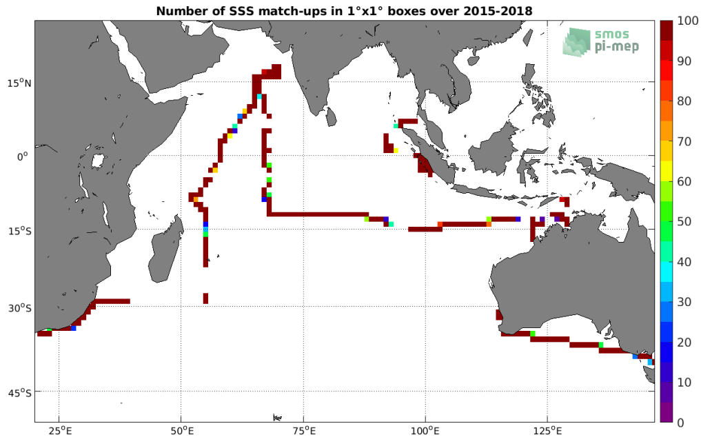
Figure 4: Number of SSS match-ups between TSG (SAMOS) SSS and the SMOS SSS L3 v2 - 9-Days (BEC) SSS product for the Indian Ocean Pi-MEP region over 1^\circ \times 1^\circ boxes and for the full satellite product period.
