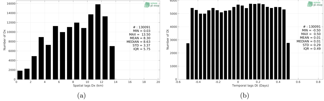
Figure 5: Histograms of the spatial (a) and temporal (b) lags between the time of the TSG (SAMOS) measurements and the date of the corresponding SMOS SSS L3 v2 - 9-Days (BEC) SSS product.
