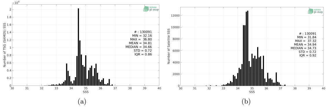
Figure 2: Histograms of SSS from TSG (SAMOS) (a) and SMOS SSS L3 v2 - 9-Days (BEC) (b) considering all match-up pairs per bins of 0.1 over the Indian Ocean Pi-MEP region and for the full satellite product period.
