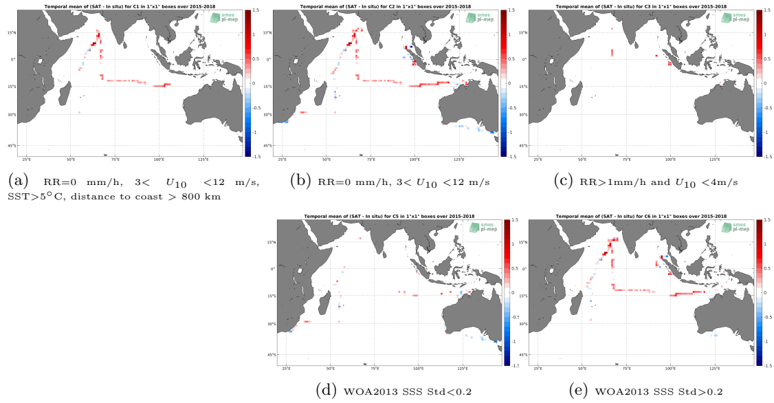
Figure 12: Temporal mean gridded over spatial boxes of size 1^\circ \times 1^\circ of \Delta SSS (SMOS SSS L3 v2 - 9-Days (BEC) - TSG (SAMOS)) for 5 different subdatasets corresponding to: RR=0 mm/h, 3 < U_{10} < 12 m/s, SST > 5^\circ C , distance to coast > 800 km (a), RR=0 mm/h, 3 < U_{10} < 12 m/s (b), RR > 1 mm/h and U_{10} < 4 m/s (c), WOA2013 SSS Std < 0.2 (d), WOA2013 SSS Std > 0.2 (e).
