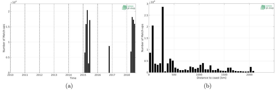
Figure 1: Number of match-ups between TSG (SAMOS) and SMOS SSS L3 v2 - 9-Days (BEC) SSS as a function of time (a) and as function of the distance to coast (b) over the Indian Ocean Pi-MEP region and for the full satellite product period.
