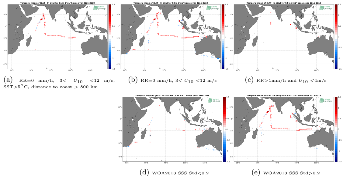
Figure 12: Temporal mean gridded over spatial boxes of size 1^\circ \times 1^\circ of \Delta SSS (SMOS L3 v2 - 9-Days (BEC) - TSG (SAMOS)) for 5 different subdatasets corresponding to: RR=0 mm/h, 3 < U_{10} < 12 m/s, SST > 5^\circ C , distance to coast > 800 km (a), RR=0 mm/h, 3 < U_{10} < 12 m/s (b), RR > 1 mm/h and U_{10} < 4 m/s (c), WOA2013 SSS Std < 0.2 (d), WOA2013 SSS Std > 0.2 (e).
