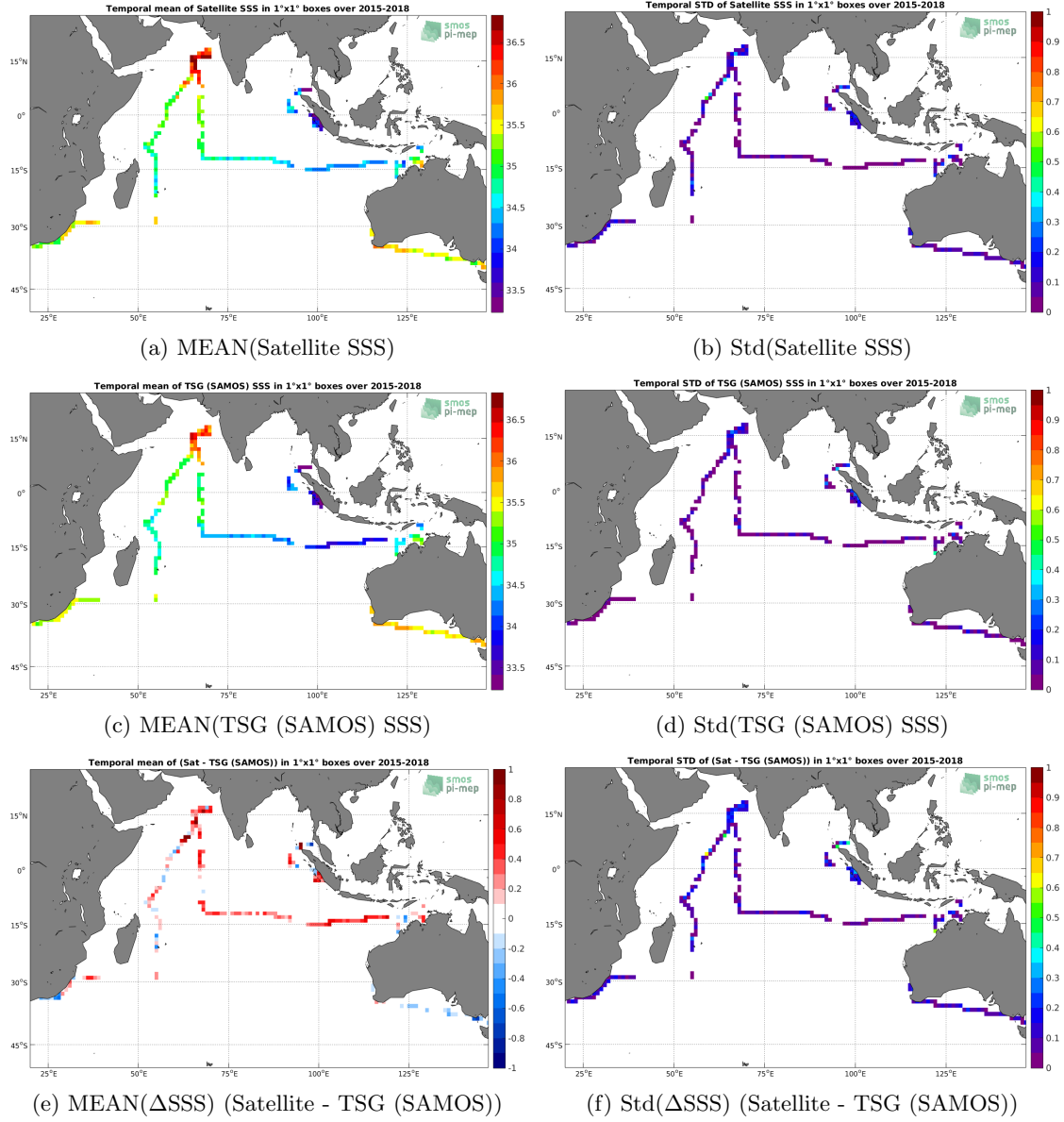
Figure 6: Temporal mean (left) and Std (right) of SSS from SMOS L3 v2 - 9-Days (BEC) (top), TSG (SAMOS) (middle), and of \Delta SSS (Satellite - TSG (SAMOS)). Only match-up pairs are used to generate these maps.
