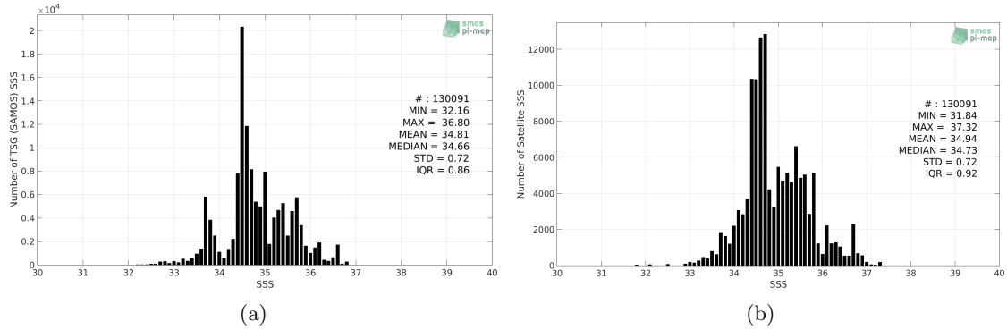
Figure 2: Histograms of SSS from TSG (SAMOS) (a) and SMOS L3 v2 - 9-Days (BEC) (b) considering all match-up pairs per bins of 0.1 over the Indian Ocean Pi-MEP region and for the full satellite product period.
