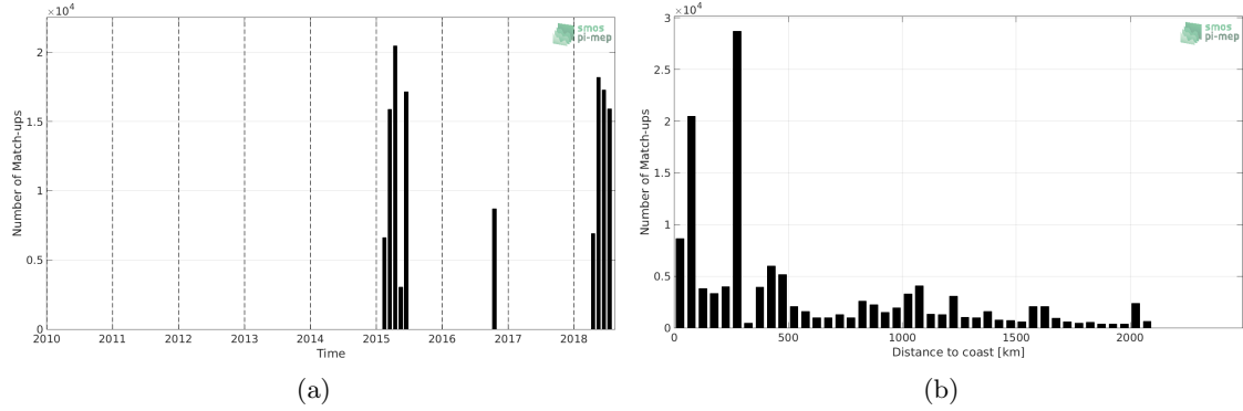
Figure 1: Number of match-ups between TSG (SAMOS) and SMOS L3 v2 - 9-Days (BEC) SSS as a function of time (a) and as function of the distance to coast (b) over the Indian Ocean Pi-MEP region and for the full satellite product period.
