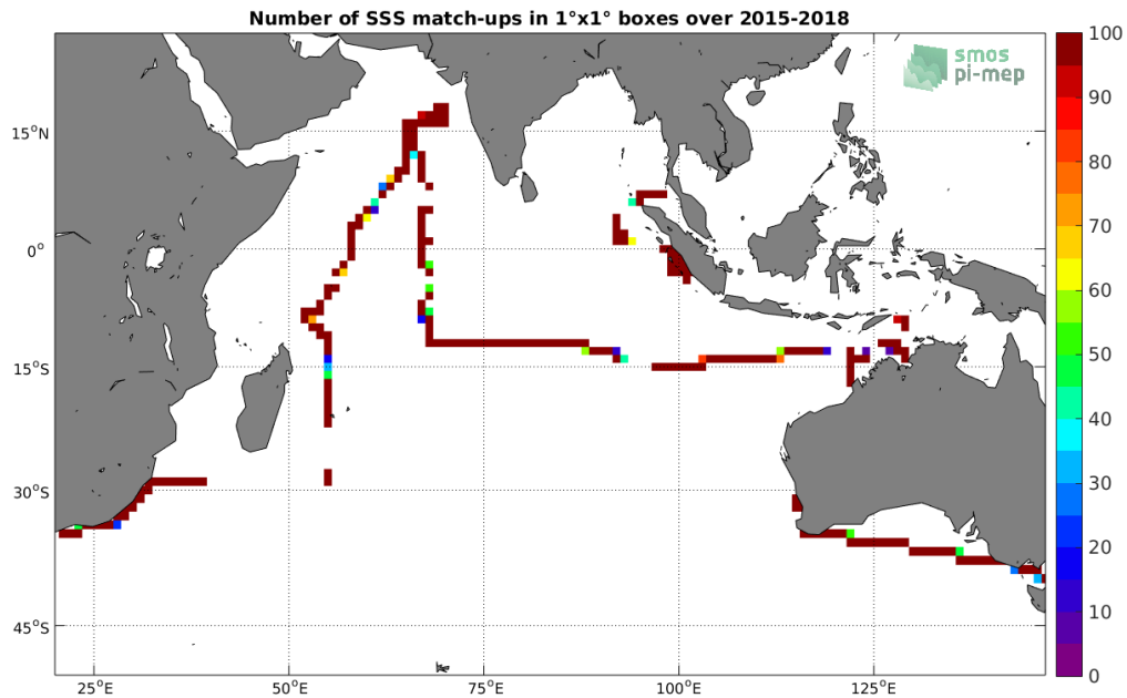
Figure 4: Number of SSS match-ups between TSG (SAMOS) SSS and the SMOS L3 v2 - 9-Days (BEC) SSS product for the Indian Ocean Pi-MEP region over 1°x1° boxes and for the full satellite product period.
