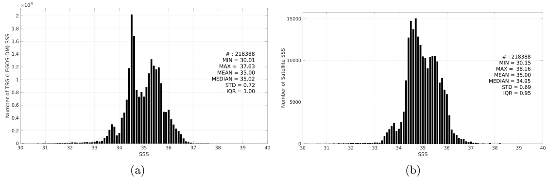
Figure 3: Histograms of SSS from TSG (LEGOS-DM) (a) and SMOS SSS L3 v2 - 9-Days (BEC) (b) considering all match-up pairs per bins of 0.1 over the Indian Ocean Pi-MEP region and for the full satellite product period.
