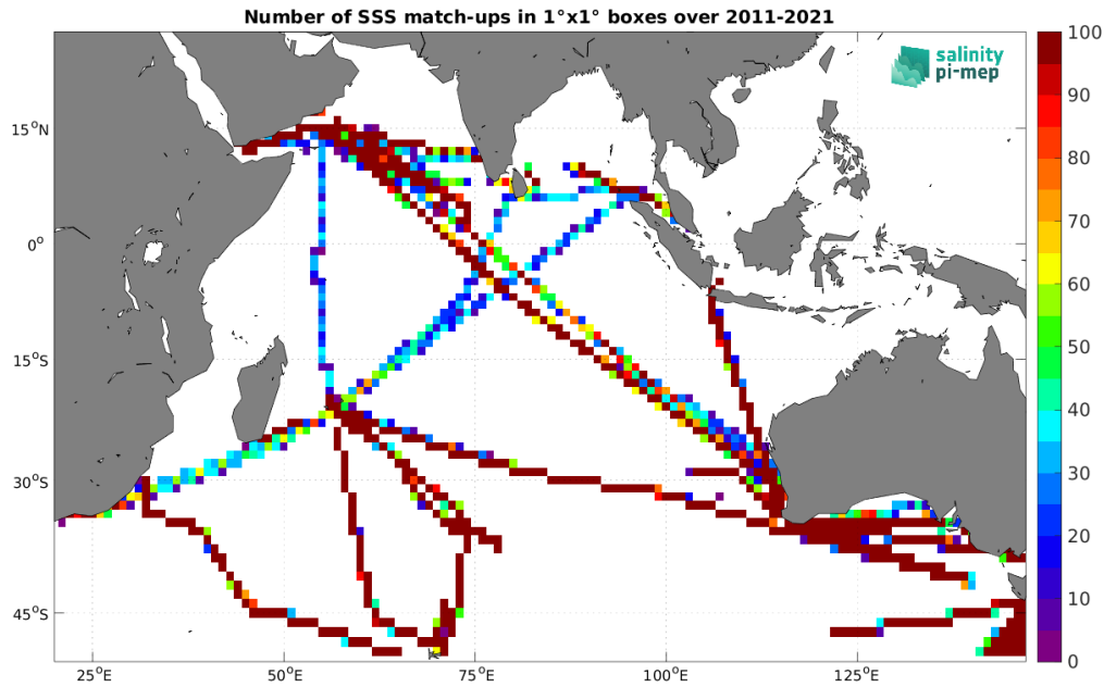
Figure 5: Number of SSS match-ups between TSG (LEGOS-DM) SSS and the SMOS SSS L3 v2 - 9-Days (BEC) SSS product for the Indian Ocean Pi-MEP region over 1^\circ \times 1^\circ boxes and for the full satellite product period.
