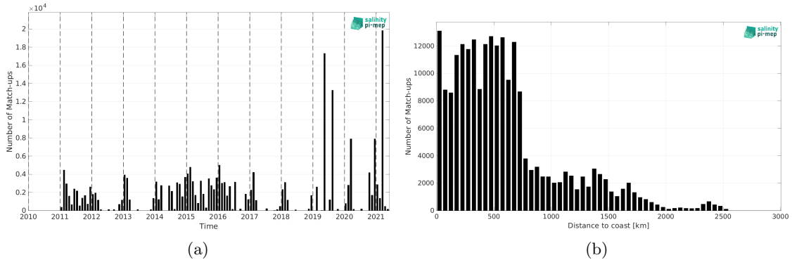
Figure 2: Number of match-ups between TSG (LEGOS-DM) and SMOS SSS L3 v2 - 9-Days (BEC) SSS as a function of time (a) and as function of the distance to coast (b) over the Indian Ocean Pi-MEP region and for the full satellite product period.
